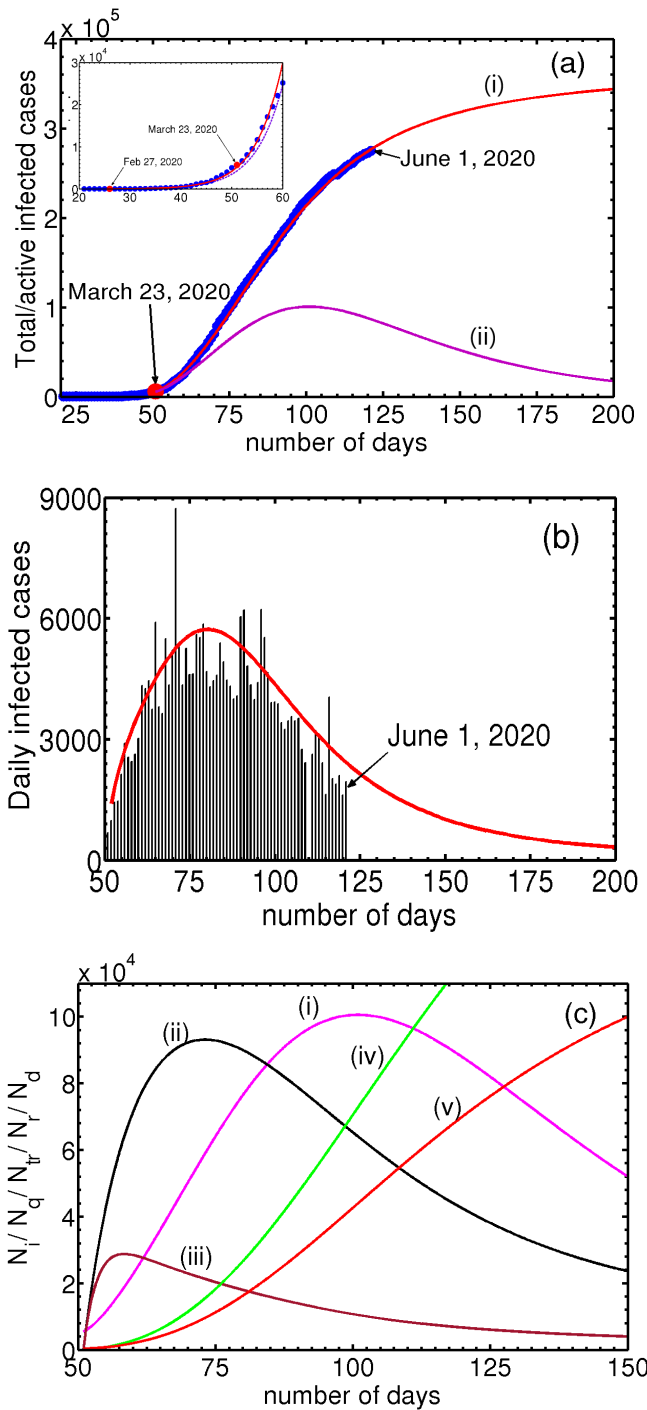
FIG. 3. (a) Inset: Plot of the total infected population (continuous curve), along with the UK data ( \bullet ) from February 27, 2020 till March 31. Also shown is the active infected N_i (dotted curve). Post Lock-down period: Plots of the total infected population (curve marked i) along with the corresponding data for the UK ( \bullet ) from March 23, 2020. Curve marked (ii) shows the active infected population. (b) Plots of the reported daily new cases for the UK along with the model predicted daily new cases. (c) Plots of the infected (i), quarantined (ii), traced (iii), recovered (iv) and deceased (v), starting from March 23, 2020. The values of the parameters used are given in Table II.
