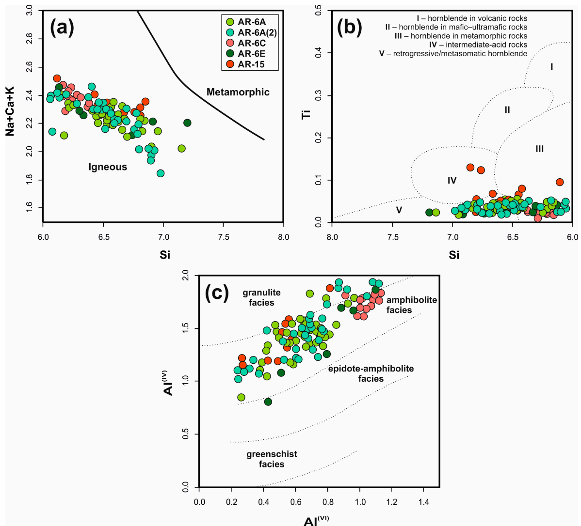
Figure 8. Discrimination diagrams for hornblendes from the Aravalli area ortoamphibolites. (a) Na + Ca + K vs. Si diagram, (b) Si vs. Ti diagram for hornblendes after [36], (c) Al^{(VI)} vs. Al^{(IV)} diagram after [37].
