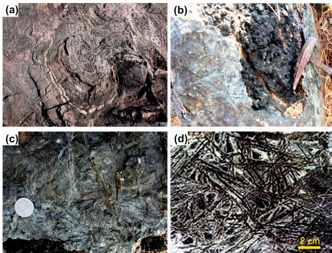
Figure 2. Field photographs showing morphology of the pillow lava outcrops at the Aravalli area. (a) pillow structures showing deformation, (b) oval shape of the pillow lava in the Aravalli area with visible spinifex-like texture on the surface, (c,d) fibrous and platy amphibole on the Aravalli pillow lava surface. Note the hammer and the coin for scale.
