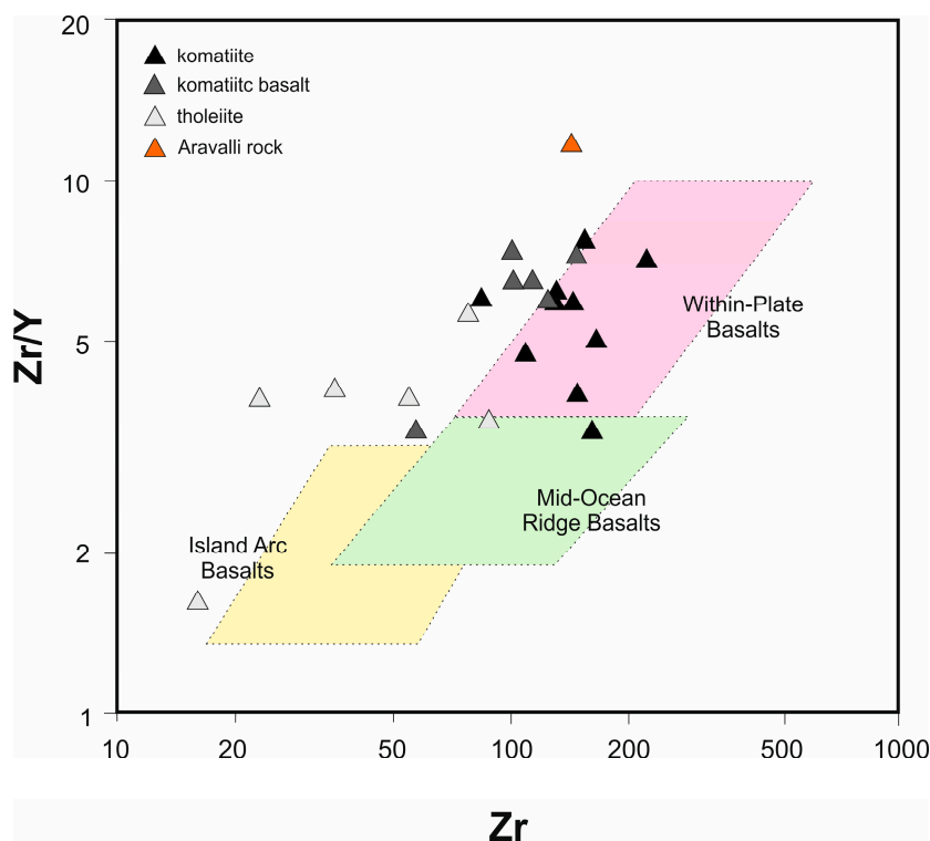
Figure 12. Zr/Y vs. Zr diagram after [46].
