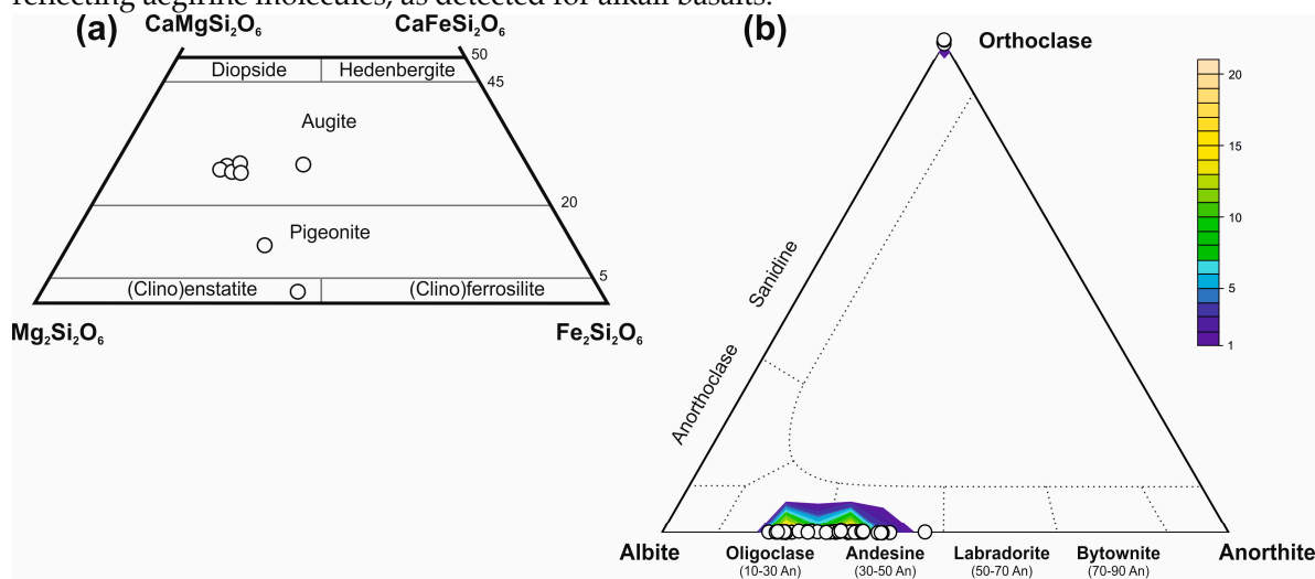
Figure 6. (a) pyroxene chemistry of the orthoamphibolites from the Aravalli area, plot of the EPMA data in the pyroxene classification diagram after [20], (b) plagioclase chemistry of the orthoamphibolites from the Aravalli area, plot of the EMPA data in the feldspar classification diagram.
