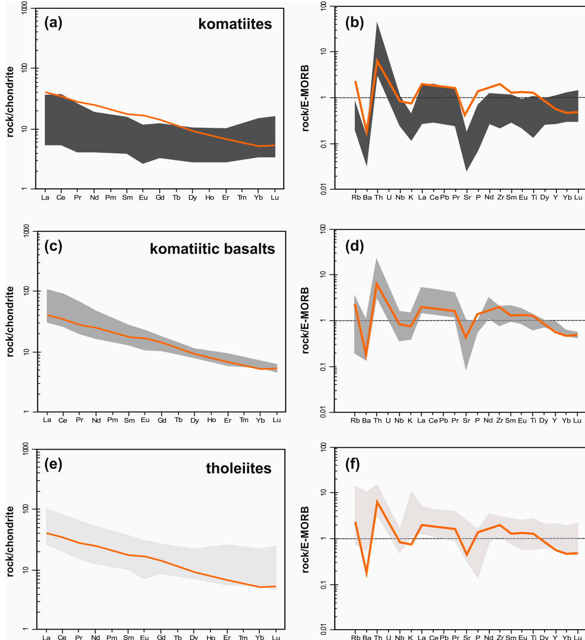
Figure 11. (a,c,e) chondrite-normalized REE patterns for komatiite, komatiitic basalts and tholeiite respectively (normalizing values after [43]), (b,d,f) E-MORB normalized multi-element spider diagrams (normalizing values after [44]) for the komatiite, komatiitic basalts and tholeiite respectively (data from [10]), REE and multi-element patterns of AR-6C (brown line) shown for comparison.
