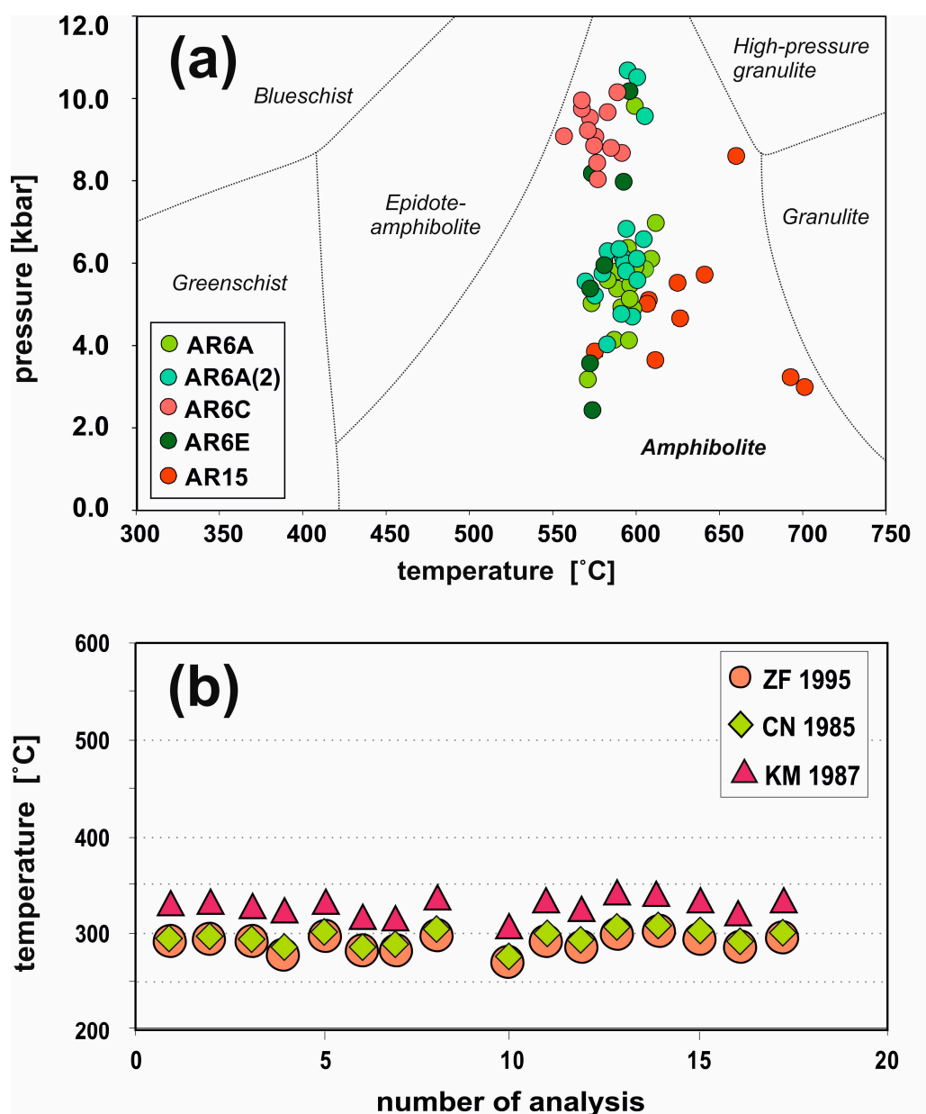
Figure 7. (a) P-T condition estimation after [29,32] (b) pressure and temperature conditions of metamorphic processes calculated on chlorite formation conditions after ZF [38], KM [39] and CN [40].
