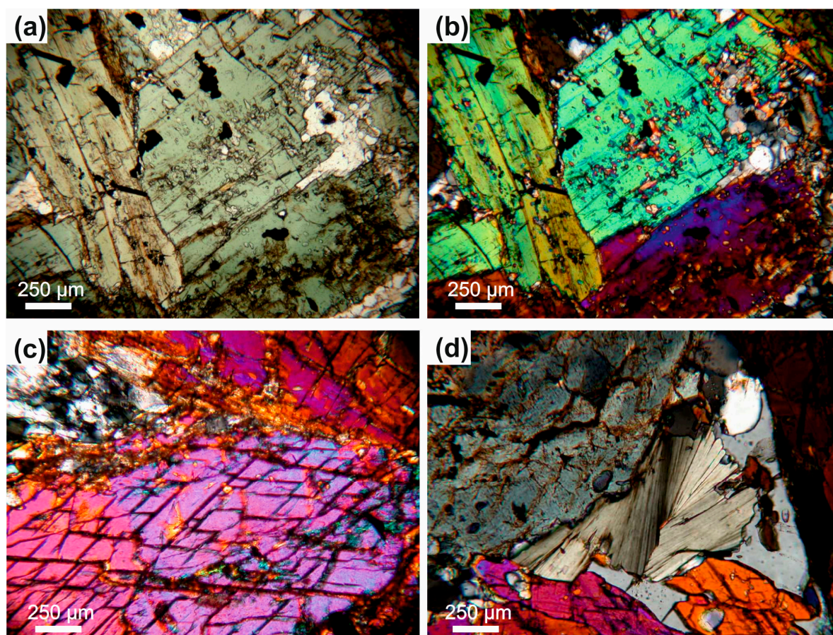
Figure 3. Photomicrographs of the studied samples from the Aravalli area. (a–c) pseudomorphic large Ca-amphibole grains making spinifex-like texture in Aravalli pillow lava, (d) retrogressive Mg chlorite after amphibole.
