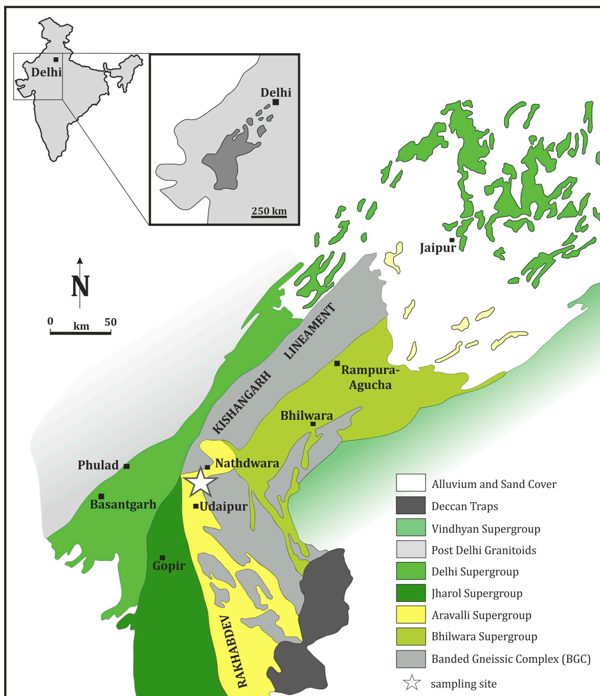
Figure 1. Simplified regional geological map of the Aravalli–Delhi orogeny after [20].
