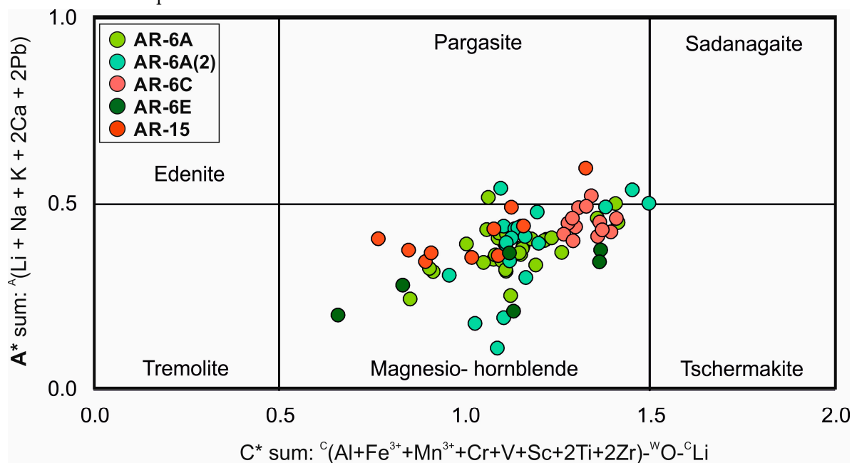
Figure 5. Ca-amphiboles chemistry from the ortoamphibolites from the Aravalli. Plot of the EMPA data in the calcic amphibole classification diagram [23]. A* ^A(Li + Na + K + 2Ca + 2Pb) ; C* ^C(Al + Fe^{3+} + Mn^{3+} + Cr + V + Sc + 2Ti + 2Zr) - ^WO - ^CLi .
