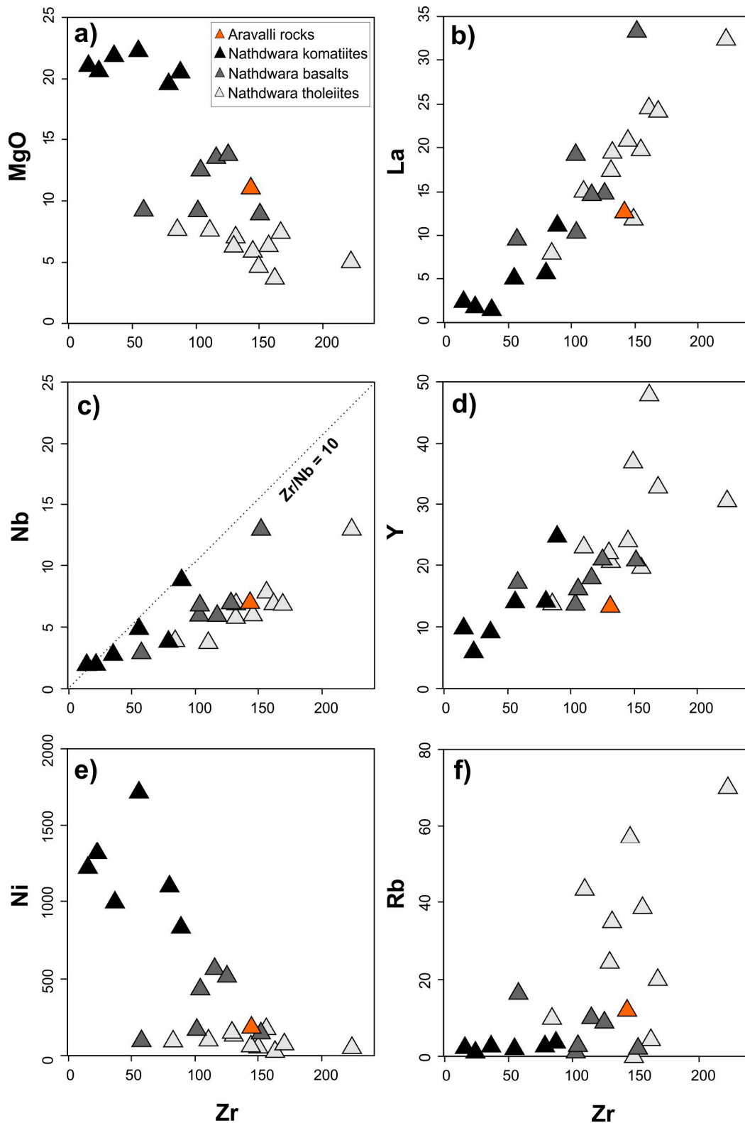
Figure 10. Bivariate plots of Zr (as an index of fractionation) versus selected elements for the AR-6C sample and Nathdwara rocks (data from [10]).
