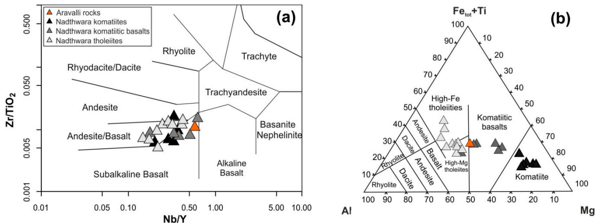
Figure 9. (a) Zr/TiO 2 vs Nb/Y plot after [41], (b) Al-(Fe tot + Ti)-Mg diagram after [42] for the AR-6C sample and Nadthwara volcanic rocks (data from [10]).
