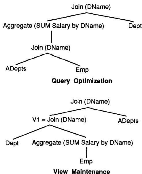
Figure 3: Query optimization versus view maintenance
