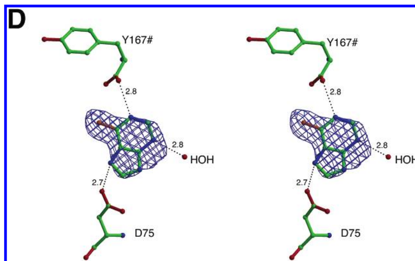
FIGURE 2: Stereoview of the active site of PTD. (A) The F_o - F_c density for the substrate dAdo is shown contoured at 3.1\sigma . (B) The F_o - F_c density for the ribosylated ester intermediate covalently bound to Glu101 is shown contoured at 3.4\sigma . (C) The F_o - F_c density for seleninosine is shown contoured at 2.9\sigma . (D) The F_o - F_c density for bromopurine is shown contoured at 3.0\sigma . This figure was prepared using BOBSCRIPT (29, 30) and Raster3D (27, 28).
