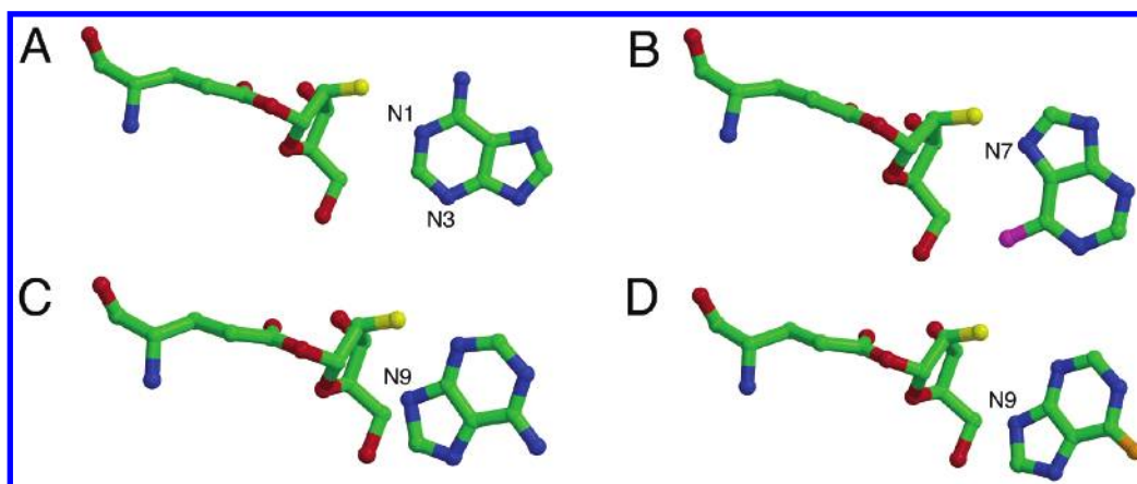
FIGURE 6: Different orientations of the purine base in the PTD active site. The four panels show the purine base and hydrogen bonding schemes for (A) the ribosylated intermediate with bound adenine, (B) 6-bromopurine, (C) deoxyadenosine, and (D) 6-seleninosine. Panels B–D show the ribosylated intermediate from panel A for reference. This figure was prepared using MOLSCRIPT (26) and Raster3D (27, 28).
