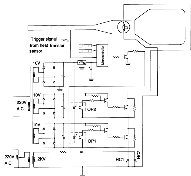
Figure 1. Schematic diagram of the hypersonic shock tunnel HST2 with the electrical circuit for flow visualization.
