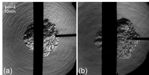
FIG. 8: NONEL 30 mm from the plates' surface, porosity (a) 9.7%, (b) 0.7%.
