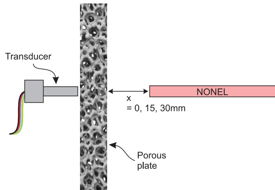
FIG. 5: Experimental setup for the measurement of total pressure behind the porous plates.
