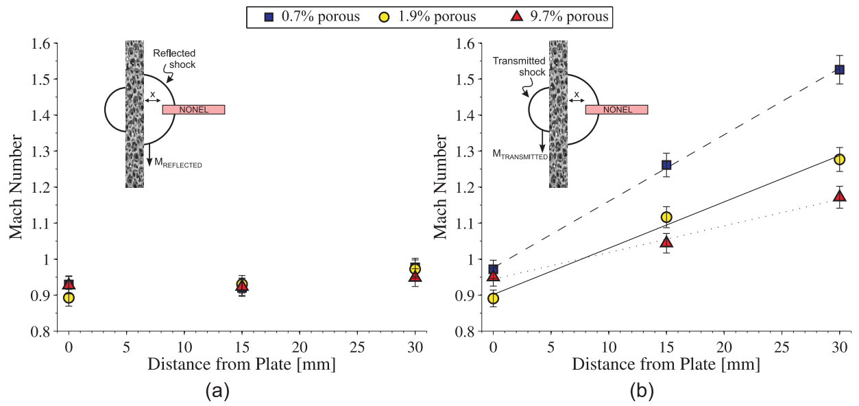
FIG. 10: Shock propagation Mach numbers along the plate surface for: (a) reflected shock, (b) transmitted shock.
