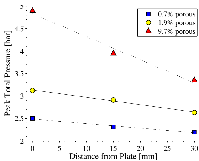
FIG. 9: Peak pressure measured after the porous plate.
