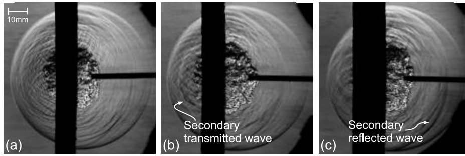
FIG. 7: NONEL 15 mm from the plates' surface, porosity (a) 9.7%, (b) 1.9%, (c) 0.7%.
