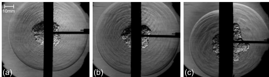
FIG. 6: NONEL flushed with the plates' surface, porosity (a) 9.7%, (b) 1.9%, (c) 0.7%.
