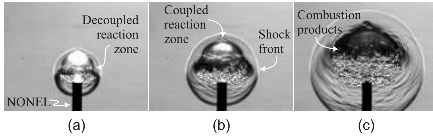
FIG. 2: Flow created by the NONEL at t = (a) 18 \mu\text{s} , (b) 30 \mu\text{s} , (c) 52 \mu\text{s} after the initial emergence of the shock front.
