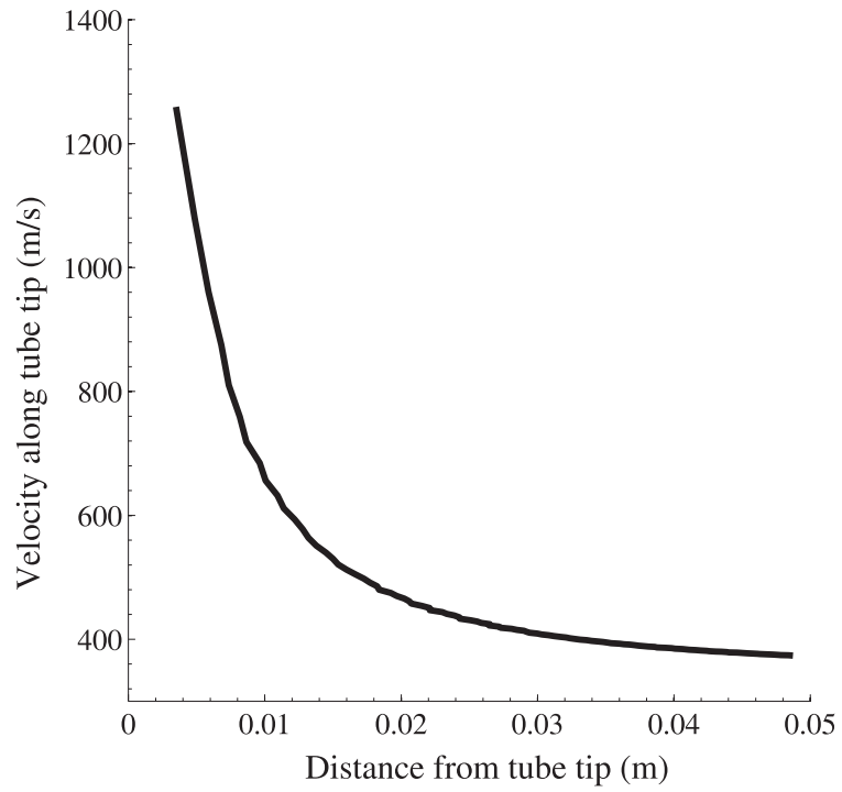
FIG. 4: Primary shock wave velocity.
