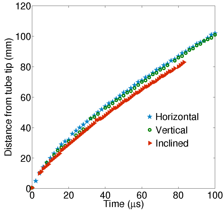
FIG. 3: Position of the shock front traced from three different vantage points.
