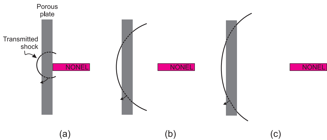
FIG. 11: Emergence of the transmitted shock at different NONEL locations: (a) flushed, (b) 15 mm, (c) 30 mm.
