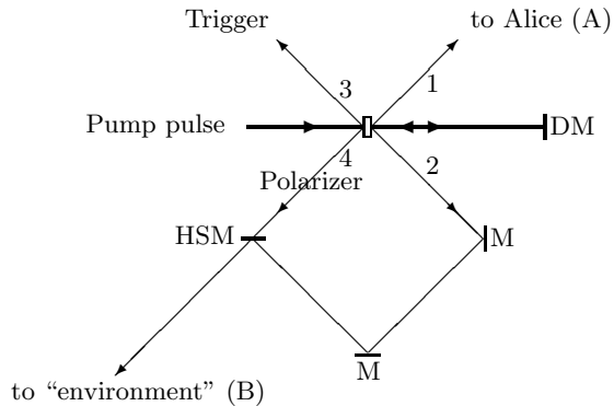
FIG. 2: Schematic description of the arrangement in the case of cloning. The down conversion crystal is denoted as a box, and delay mirror, mirrors, and half-silvered mirror are denoted respectively by DM, M, and HSM. See text for details.
