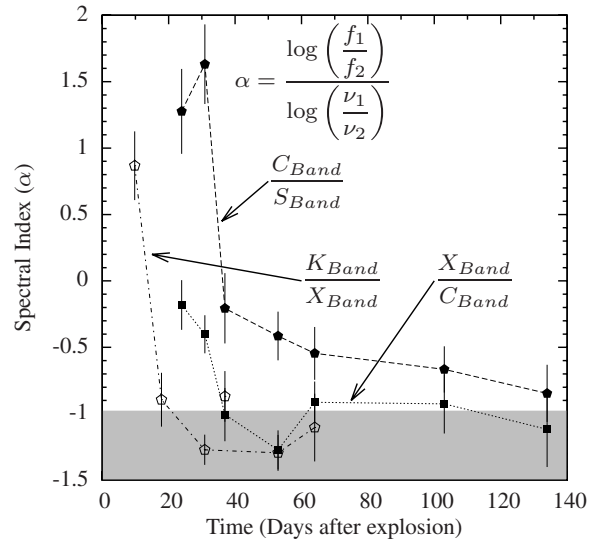
Figure 1. Spectral-index curves made using the S-, C-, X-, and K-band data. In case of the X_{\text{Band}}/C_{\text{Band}} and K_{\text{Band}}/X_{\text{Band}} ratios, the spectral-index values are smaller than -1 for an extended period of time between 20 and 60 days. The C_{\text{Band}}/S_{\text{Band}} index approaches the optically thin value slowly as the SN ages. The spectral indices calculated from higher frequency bands show observable deviations due to cooling of the relativistic electrons.
