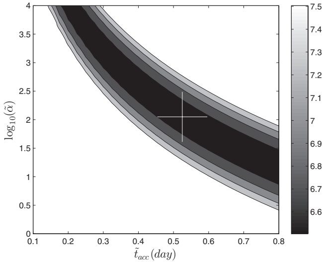
Figure 8. Calculated \chi^2 as a function of \tilde{t}_{\text{acc}} and equipartition factor ( \log_{10} \tilde{\alpha} ) for t_{\text{ff}} = 18.5 days using Model-4 (refer to Table 2) with the explosion date 2012 March 15.3 UT. The cross represents the best fit values of \tilde{t}_{\text{acc}} and \tilde{\alpha} with \chi^2 \sim 6.50 . The grayscale shows the value of \chi^2 and the corresponding contours. The levels marked in the contour plot are separated by \sim 0.2 . For Compton cooling to be dominant, we need \tilde{\alpha} > 1.0 , therefore the region below \log_{10}(\tilde{\alpha}) < 0.0 is rejected. The best fit parameters of this model are given in Table 2.
