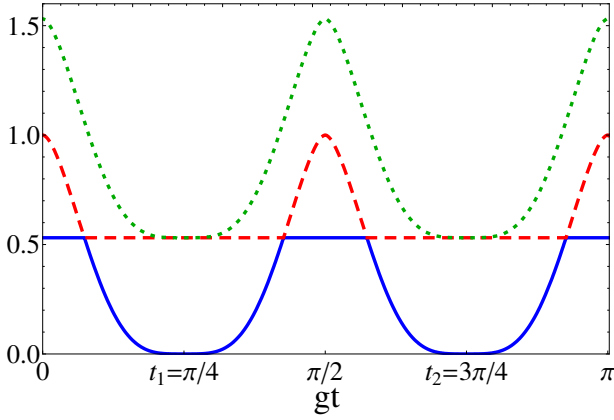
FIG. 11: Dynamics of quantum discord \mathcal{D} (blue solid line), classical correlation J (red dashed line) and total correlation I (green dotted line) for an initial Bell-diagonal state of the form \rho_{AB}(0) = \lambda_1(0)|\psi^+\rangle\langle\psi^+| + \lambda_2(0)|\psi^-\rangle\langle\psi^-| + \lambda_3(0)|\phi^+\rangle\langle\phi^+| + \lambda_4(0)|\phi^-\rangle\langle\phi^-| with \lambda_1(0) = 0.9 , \lambda_2(0) = 0.1 and \lambda_3(0) = \lambda_4(0) = 0 , passing through local channels, with each channel being modeled by an interaction between the corresponding qubit and a classical field. The interaction strength is given by g\hbar . The vertical axis is in bits while the horizontal axis is dimensionless. [Reprinted from Ref. [640] with permission. Copyright 2012 American Physical Society.]
