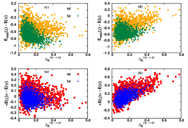
FIG. 8. (Color Online.) Quantifying cost-efficient catalysts. \langle E(\chi) \rangle - E(\psi) (in (a)) and \langle E(\chi) \rangle - E(\phi) (in (b)) (ordinate) against the single-copy entanglement difference, \Delta_E^{\psi \rightarrow \phi} (abscissa). Squares and triangles represent the Haar uniformly generated states in 4 \otimes 4 and 5 \otimes 5 respectively. (c) and (d) Similar plots as in (a) and (b) where the vertical axis is for E_{min}(\chi) - E(\psi) and E_{min}(\chi) - E(\phi) in (c) and (d) respectively. Circles and diamonds correspond to 4d and 5d catalyst states. All the axes are dimensionless.
