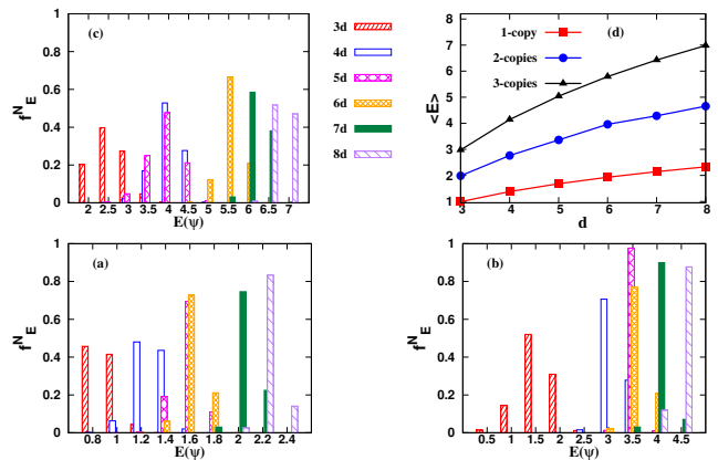
FIG. 1. (Color Online.) Entanglement patterns of random pure bipartite states in d \otimes d . The normalized frequency distribution of entanglement (quantified by entanglement entropy), f_E^N (ordinate) is shown against E(\psi) (abscissa) for (a) 1-copy, (b) 2-copies and (c) 3-copies. (d) Mean entanglement, \langle E \rangle (ordinate) with respect to the dimension, d (abscissa) for 1-copy (bottom line with squares), 2-copies (middle line with circles) and 3-copies (top line with triangles). We Haar uniformly simulate 10^6 states in each dimension. All the axes are dimensionless.
