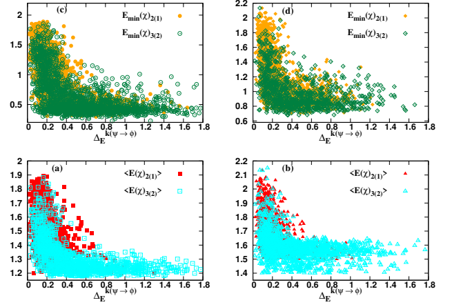
FIG. 5. (Color Online.) Entanglement patterns of one step-assisted catalysts. (a) \langle E(\chi)_{2(1)} \rangle (solid squares) and \langle E(\chi)_{3(2)} \rangle (hollow squares) (ordinate) with respect to \Delta_E^{k(\psi \rightarrow \phi)} (abscissa) having k = 1, 2 respectively for randomly generated states in 4 \otimes 4 . (c) The similar plot as in (a) for E_{\min}(\chi)_{2(1)} (solid circles) and E_{\min}(\chi)_{3(2)} (hollow circles). (b) and (d) are for random states in 5 \otimes 5 . (b) is similar to (a) with squares being replaced by triangles while (d) is similar to (c) except circles are changed to diamonds. All the axes are dimensionless.
