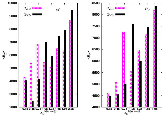
FIG. 6. (Color Online.) \langle n_\chi \rangle (ordinate) against \Delta_E^{k(\psi \rightarrow \phi)} (abscissa) with k = 1, 2 for catalysts |\chi\rangle_{2(1)} (stripes) and |\chi\rangle_{3(2)} (solid) respectively. (a) Distribution of \langle n_\chi \rangle in 4 \otimes 4 while (b) is for 5 \otimes 5 . All the axes are dimensionless.
