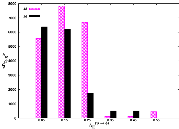
FIG. 7. (Color Online.) Frequency distribution of average number of strong catalysts , \langle n_{\chi_{3(1)}} \rangle (ordinate) with \Delta_E^{\psi \rightarrow \phi} (abscissa) for 3-copy incomparable states found in 4 \otimes 4 (stripes) and 5 \otimes 5 (solid). Unlike one step-assisted catalysts, they can be found in good numbers for low values of \Delta_E^{\psi \rightarrow \phi} . All the axes are dimensionless.
