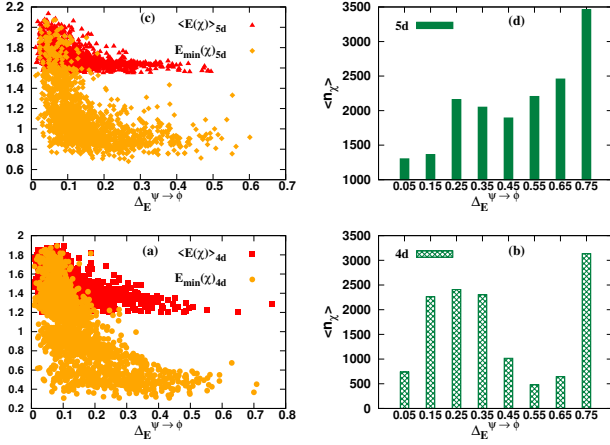
FIG. 3. (Color Online.) (a) Mean entanglement, \langle E(\chi) \rangle (squares) and minimum entanglement, E_{min}(\chi) (circles) of catalyst states (ordinate) vs. \Delta_E^{\psi \rightarrow \phi} (abscissa) when random states with E(\psi) \geq E(\phi) are used to check incomparability as well as for catalysts in 4 \otimes 4 . (c) Triangles and diamonds represent \langle E(\chi) \rangle and E_{min}(\chi) respectively in 5 \otimes 5 . (b) and (d) The average number of catalyst states, \langle n_\chi \rangle against \Delta_E^{\psi \rightarrow \phi} (abscissa) for random states in 4d (striped columns) (in (b)) and 5d (solid columns) (in (d)). In all the plots, states are incomparable when a single copy of the input-target pair is available. The data is computed by generating 5 \times 10^4 pairs to find incomparable states while for a given incomparable pair, 10^5 catalysts are simulated. All the axes are dimensionless.
