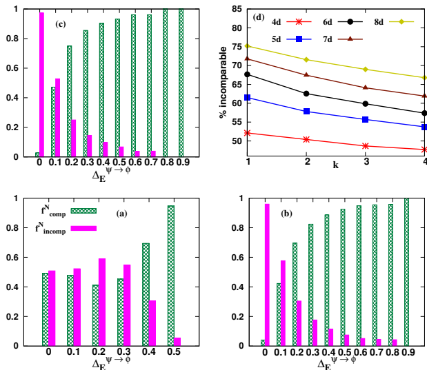
FIG. 2. (Color Online.) Incomparable vs. comparable states. (a)-(c) Normalized frequency distributions of incomparable f_{incomp}^N (solids) and comparable states, f_{comp}^N (stripes) (vertical axis) vs. \Delta_E^{\psi \rightarrow \phi} (horizontal axis) when 10^6 states are generated Haar uniformly with E(\psi) \geq E(\phi) in 3 \otimes 3 (a), 4 \otimes 4 (b) and 5 \otimes 5 (c). (In short, d \otimes d is referred to as dd systems.) (d) The percentage of incomparable bipartite states (ordinate) with respect to the number of copies k (abscissa) in 4d (red stars), 5d (blue squares), 6d (black circles), 7d (brown triangles) and 8d (yellow diamonds). All the axes are dimensionless.
