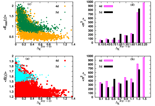
FIG. 4. (Color Online.) (a) \langle E(\chi) \rangle of catalysts for 2-copy incomparable states (ordinate) in 4d (squares) and 5d (triangles) with respect to \Delta_E^{2(\psi \rightarrow \phi)} (abscissa). (c) The same as in (a) except the ordinate is for E_{\min}(\chi) (circles and diamonds are used for states in 4d and 5d respectively). (b) The average number of catalysts, \langle n_\chi^2 \rangle for 2-copy incomparable states and (d) \langle n_\chi^3 \rangle for 3-copy incomparable states with 4d (stripes) and 5d (solid) (ordinate) against \Delta_E^{k(\psi \rightarrow \phi)} with k = 2 in (b) and k = 3 in (d). All the axes are dimensionless.
