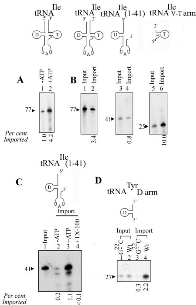
FIG. 3. Import of derivatives of tRNA Ile (UUA). (A) Import of intact tRNA Ile (UUA) into mitochondria in absence (lane 1) or presence (lane 2) of 4 mM ATP. (B) The uptakes of full-length and truncated versions of tRNA Ile (UUA) by intact mitochondria (100 μg) were compared. Left, full-length tRNA Ile (UUA); lane 1, input, 2 fmol; lane 2, 50 fmol of RNA incubated with mitochondria and assayed for import. Middle, RNA Ile (1-41); lane 3, input, 1 fmol; lane 4, 50 fmol of RNA assayed for import. Right, tRNA Ile (42-66); lane 5, input, 2 fmol; lane 6, 50 fmol of RNA assayed for import. (C) Effect of ATP on import of RNA Ile (1-41) (100 fmol). Import reactions were carried out in the absence (lane 2) or presence (lanes 3 and 4) of 4 mM ATP. After the incubation, Triton X-100 (0.5%) was added to reaction mixture 4, followed by RNase in all reaction mixtures. Lane 1, input (1 fmol). (D) Sequence-specific import of the tRNA Tyr D arm. Wild-type or G 22 →C mutant form of the D arm oligonucleotide (50 fmol) was assayed for import (lanes 4 and 3, respectively). Lanes 1 and 2, input RNA, 1 fmol. The fraction of each RNA imported is shown below the lanes.
