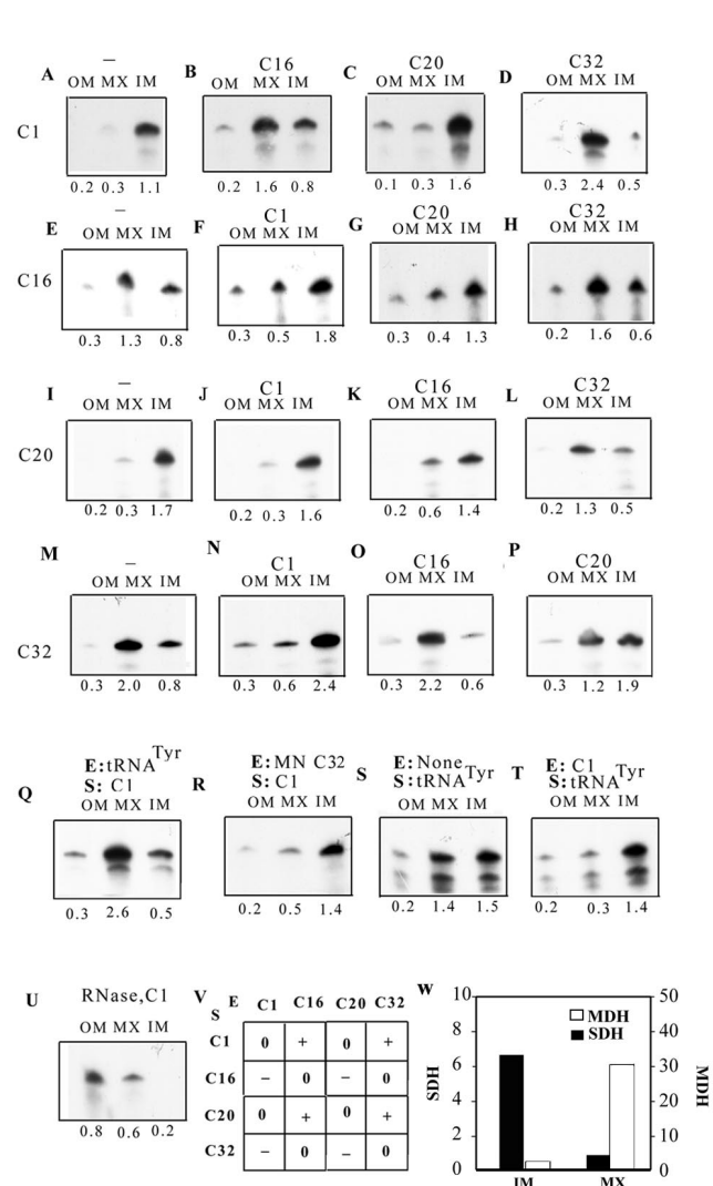
FIG. 8. Interactions between aptamers at inner membrane. Intra-mitochondrial distribution assays were performed with high-specific-activity substrate (S; 100 fmol) and low-specific-activity effector (E; 10 fmol) in the following combinations, and the RNA associated with the outer membrane plus intermembrane space (OM), inner membrane (IM), and matrix (MX) fractions was analyzed. (A) Substrate, C1, no effector; (B) substrate, C1; effector, C16; (C) substrate, C1; effector, C20; (D) substrate, C1; effector, C32; (E) substrate, C16; no effector; (F) substrate, C16; effector, C1; (G) substrate, C16; effector, C20; (H) substrate, C16; effector, C32; (I) substrate, C20; no effector; (J) substrate, C20; effector, C1; (K) substrate, C20; effector, C16; (L) substrate, C20; effector, C32; (M) substrate, C32; no effector; (N) substrate, C32; effector, C1; (O) substrate, C32; effector, C16; (P) substrate, C32; effector, C20; (Q) substrate, C1; effector, tRNA Tyr ; (R) substrate, C1; effector, micrococcal-nuclease-treated C32; (S) substrate, tRNA Tyr ; no effector; (T) substrate, tRNA Tyr ; effector, C1; (U) substrate, C1; no effector, mitoplast treated with RNase before separation of inner membrane and matrix fractions. (V) Summary of interaptamer interactions at the inner membrane. +, stimulation of inner membrane transfer; -, inhibition; 0, no significant effect. The absolute amount of RNA in each band was obtained by liquid scintillation counting; relative scan densities varied, depending on specific activities of the RNAs, exposure times of the autoradiograms, etc. (W) Specific activities (nanomoles of substrate converted/minute/miligram of protein) of succinate dehydrogenase (SDH) and malate dehydrogenase (MDH) in inner membrane and matrix fractions.
