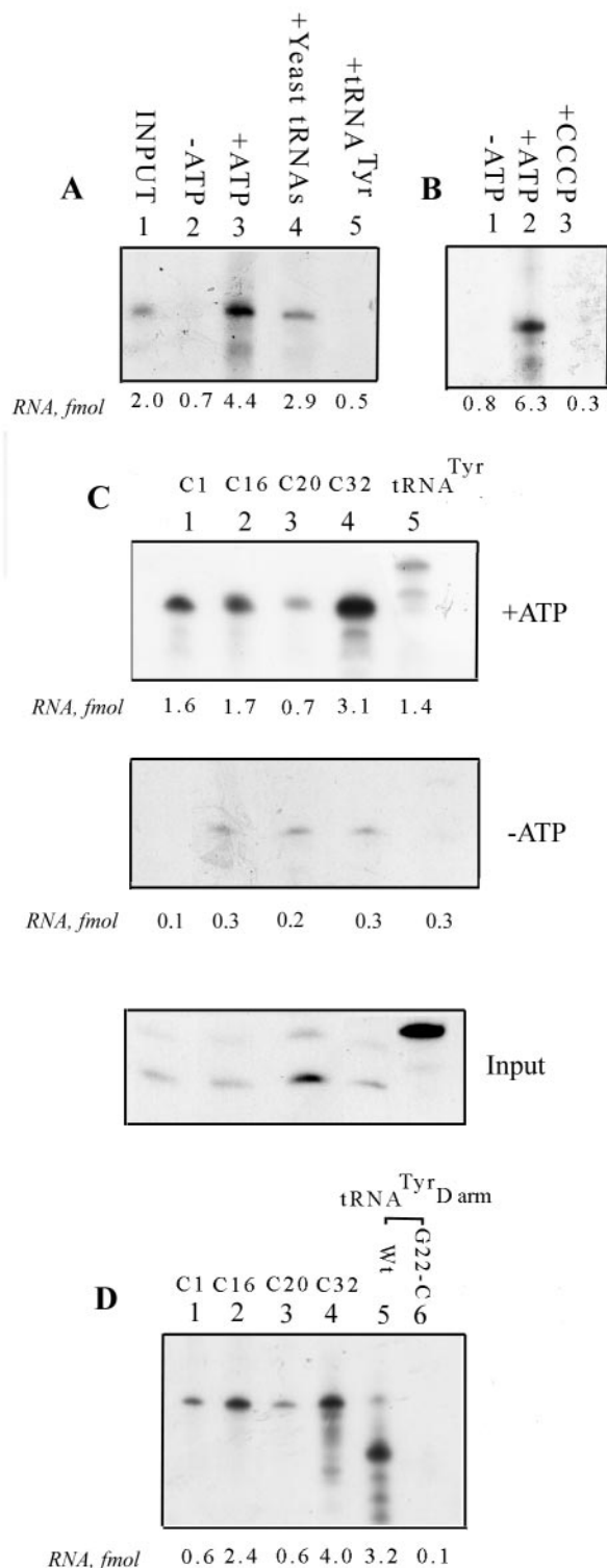
FIG. 4. In vitro import of individual aptamers. (A) Import characteristics of C32. ^{32} P-labeled C32 RNA (100 fmol) was incubated with 100 \mu g of mitochondria in the absence (lane 2) or presence (lanes 3 to 5) of 4 mM ATP for 15 min at 37°C. Lanes 4 and 5, yeast tRNA or low-specific-activity tRNA Tyr (1 pmol each) was included as competitor. (B) Mitoplast import assay. ^{32} P-labeled C32 RNA (100 fmol) was incubated with mitoplasts prepared from 100 \mu g of mitochondria in either the absence of ATP (lane 1) or presence of 4 mM ATP (lanes 2 and 3). Lane 3, 50 \mu M CCCP was included. (C) Comparison of C1, C16, C20, and C32 (lanes 1 to 4, respectively) and tRNA Tyr (lane 5) for
