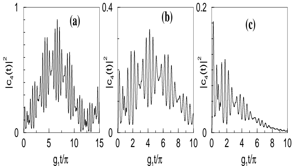
FIG. 5: Periodic behavior of two atom two photon emission probability |c_4(t)|^2 , for identical atoms interacting with vacuum in a bimodal cavity, for \delta = 3.5g_1 , \Delta = -5g_1 , g_2 = 1.5g_1 and cavity damping constants (a) \kappa_a = \kappa_b = 0.00 , (b) \kappa_a = \kappa_b = 0.03g_1 , (c) \kappa_a = \kappa_b = 0.1g_1 .
