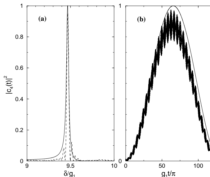
FIG. 3: The maximum value of the two atom two photon emission probability, |c_4(t)|^2 in the system of two identical atoms interacting with vacuum in a two mode cavity, is plotted with respect to (a) detuning \delta and (b) time, for g_2/g_1 = 1.5 and \Delta = -10g_1 . The solid line is corresponding to approximate result and the dotted line (...) corresponding to exact numerical result.
