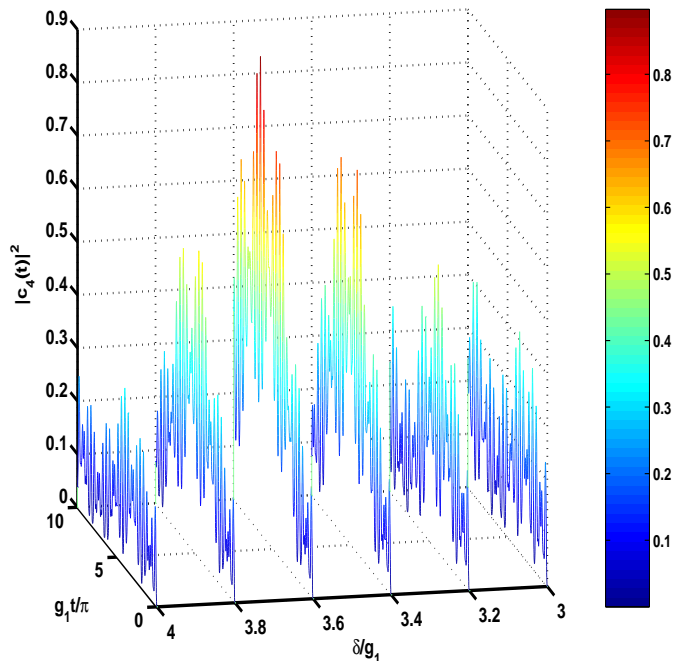
FIG. 2: (Color online) Two atom two photon emission probability, |c_4(t)|^2 in a system of identical atoms interacting with vacuum in a two mode cavity, for g_2/g_1 = 1.5 and \Delta/g_1 = -5.0 .
