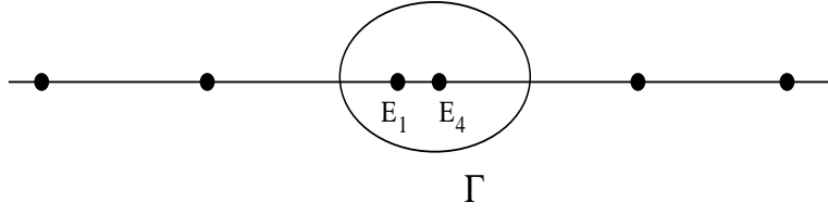
FIG. 6: The contour in complex plane shielding two eigenvalues E_1 and E_4 and leaving others outside.
