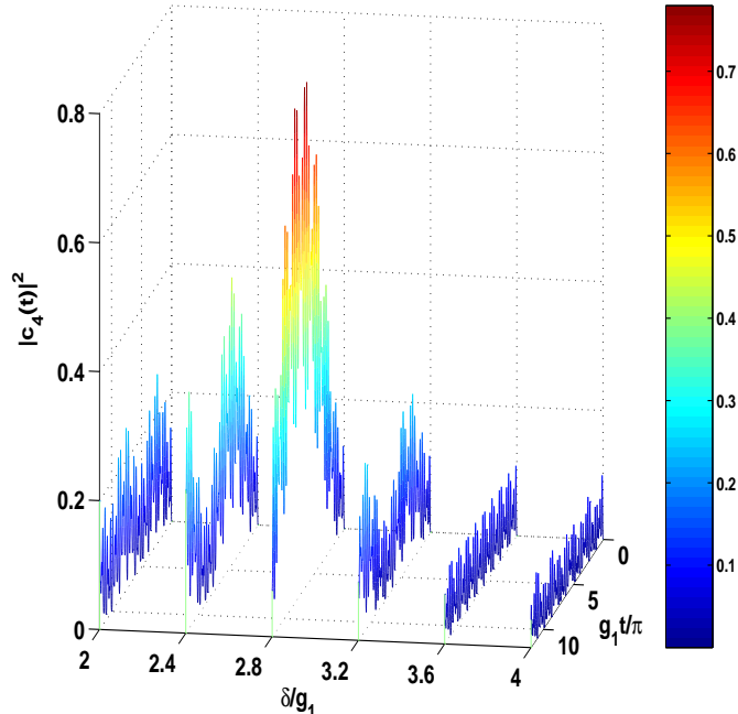
FIG. 4: (Color online) Two atom two photon emission probability, |c_4(t)|^2 in a system of nonidentical atoms interacting with vacuum in a single mode cavity, for \Delta/g_1 = -5.0 and g_2/g_1 = 2.0 .
