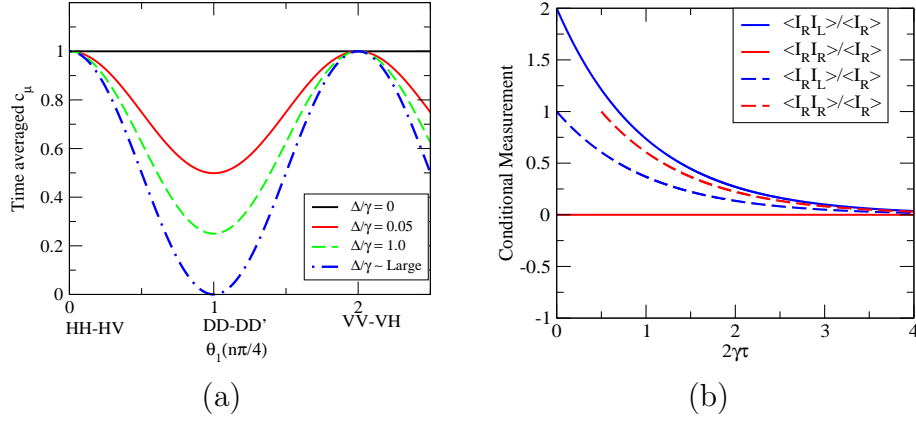
Figure 3. (Colour online) (a) Degree of correlation averaged over time as a function of basis angle, for different excitonic level splitting \Delta . H , D, D', V stands for horizontal, diagonal, orthodiagonal and vertical polarisation basis respectively. Here we have considered zero dephasing of the excitonic states. (b) Conditional measurement of intensity-intensity correlation in the circular basis. The red curve corresponds to co-polarised ( \theta_1 = \theta_2 = \pi/4, \phi_1 = \phi_2 = -\pi/2 ) photons and the blue for cross-polarised ( \theta_1 = \theta_2 = \pi/4, \phi_1 = -\pi/2, \phi_2 = \pi/2 ) ones. The solid curve is for \Delta = 0 and the broken one for \Delta \sim \text{large} . Here R and L stands for right and left circular polarisation. The R-R correlation curve in case of large splitting is time shifted for better comparison to the R-L correlation. All parameters are normalized with respect to \gamma .
