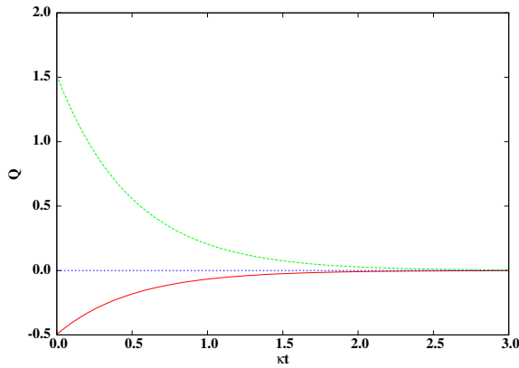
FIG. 5: Variation of the Q -parameter with time in presence of decoherence due to decay of photon for squeezing parameters r = 0.31 (red line) and r = 0.8 (green line).
