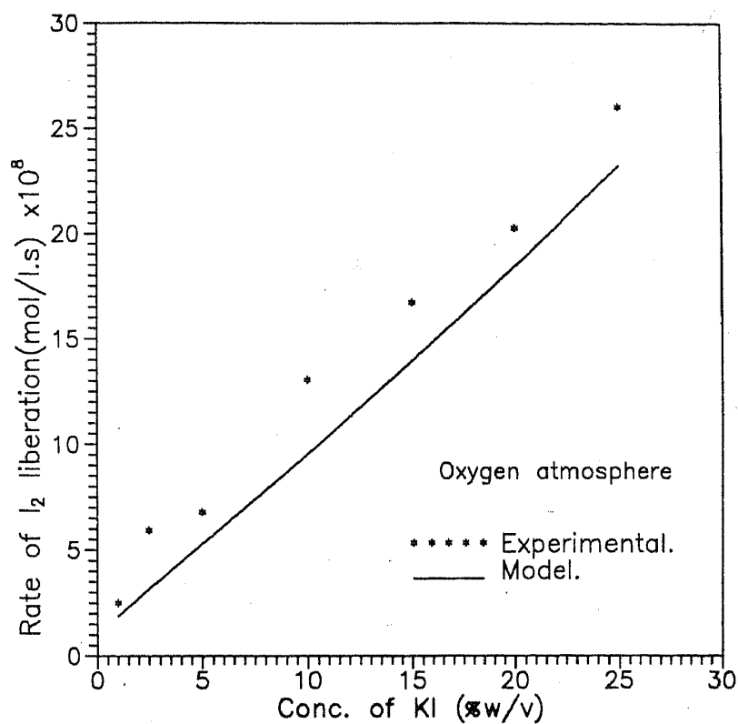
Figure 2. Comparison of model predictions with observation of iodine liberation rates: oxygen atmosphere.
