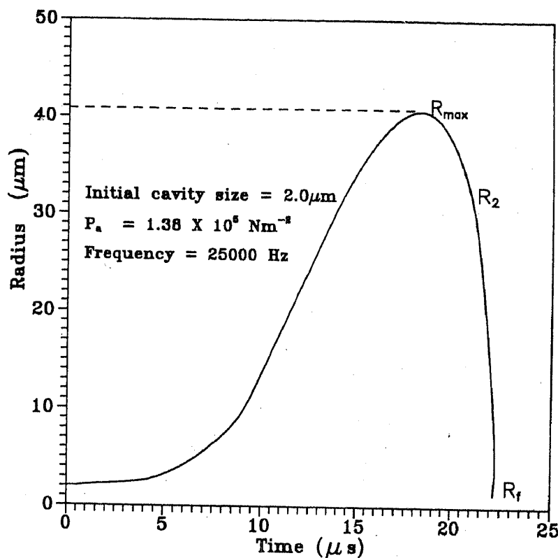
Figure 1. Curve showing typical radius versus time history.
