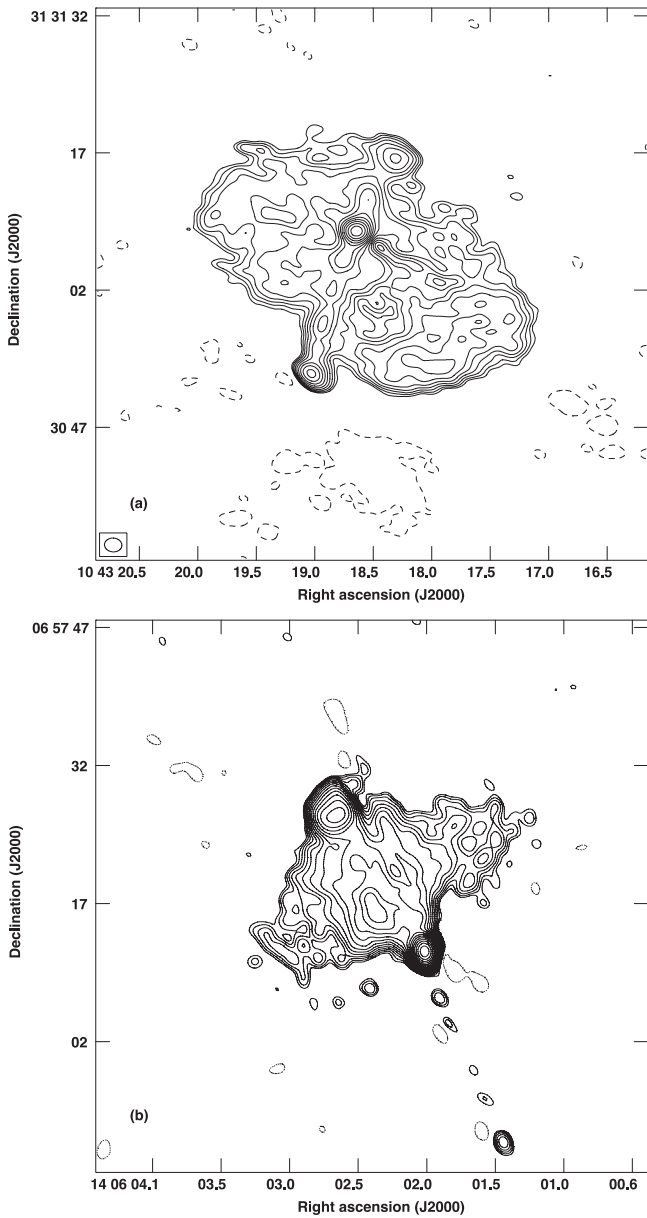
Figure 2. VLA L-band images of radio galaxies that are candidates for genuine X-shape sources created by axis reorientations. (a) The upper panel shows J1043+3131 (lowest contour = 0.3 \text{ mJy beam}^{-1} , peak = 44.6 \text{ mJy beam}^{-1} ); (b) the lower panel shows J1406+0657 (lowest contour = 0.15 \text{ mJy beam}^{-1} , peak = 71.4 \text{ mJy beam}^{-1} ).
