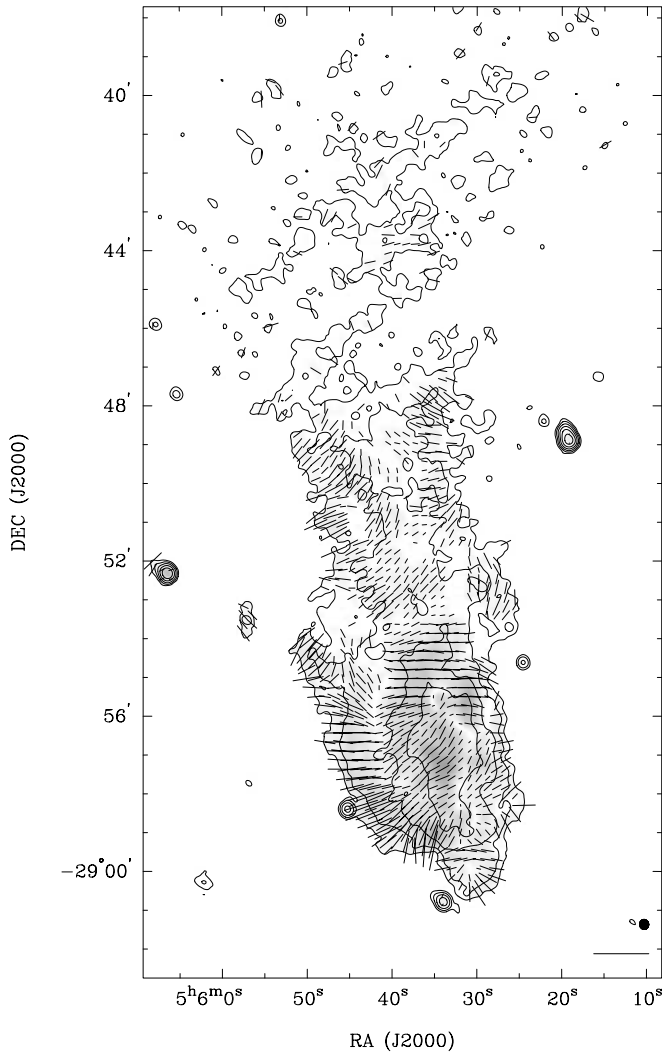
FIG. 5.—The 1520 MHz VLA image of the polarization in the emission from the southern lobe of MSH 05-22. The parameters for this image representation are the same as for Fig. 4.
