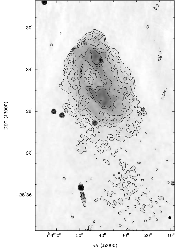
FIG. 2.—The 1520 MHz total intensity VLA image of the northern lobe of MSH 05-22. The radio image has a beam of FWHM 15.5'' \times 14.2'' at a P.A. of 8.6^\circ . Contours are at (-1, 1, 2, 3, 4, 6, 8, 12, \text{ and } 16) \times 0.4 \text{ mJy beam}^{-1} ; gray scales are over the range -0.3 to 7 \text{ mJy beam}^{-1} .
