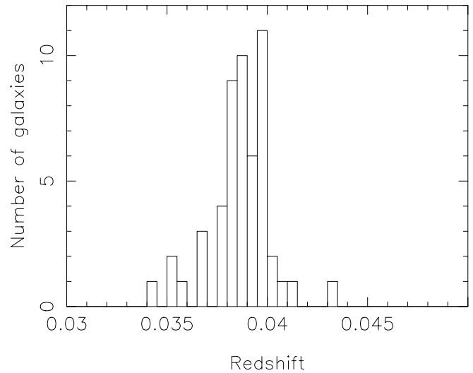
FIG. 8.—Histogram of the redshift distribution of the galaxies within 1^\circ of the host on the sky, and within the redshift range z = 0.03 – 0.05 .
