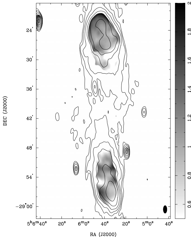
FIG. 12.—Spectral index distribution between 843 and 1520 MHz, made using images with beam FWHM 94.0'' \times 45.0'' . Gray scales span the range \alpha = -0.5 to -2.0 .
