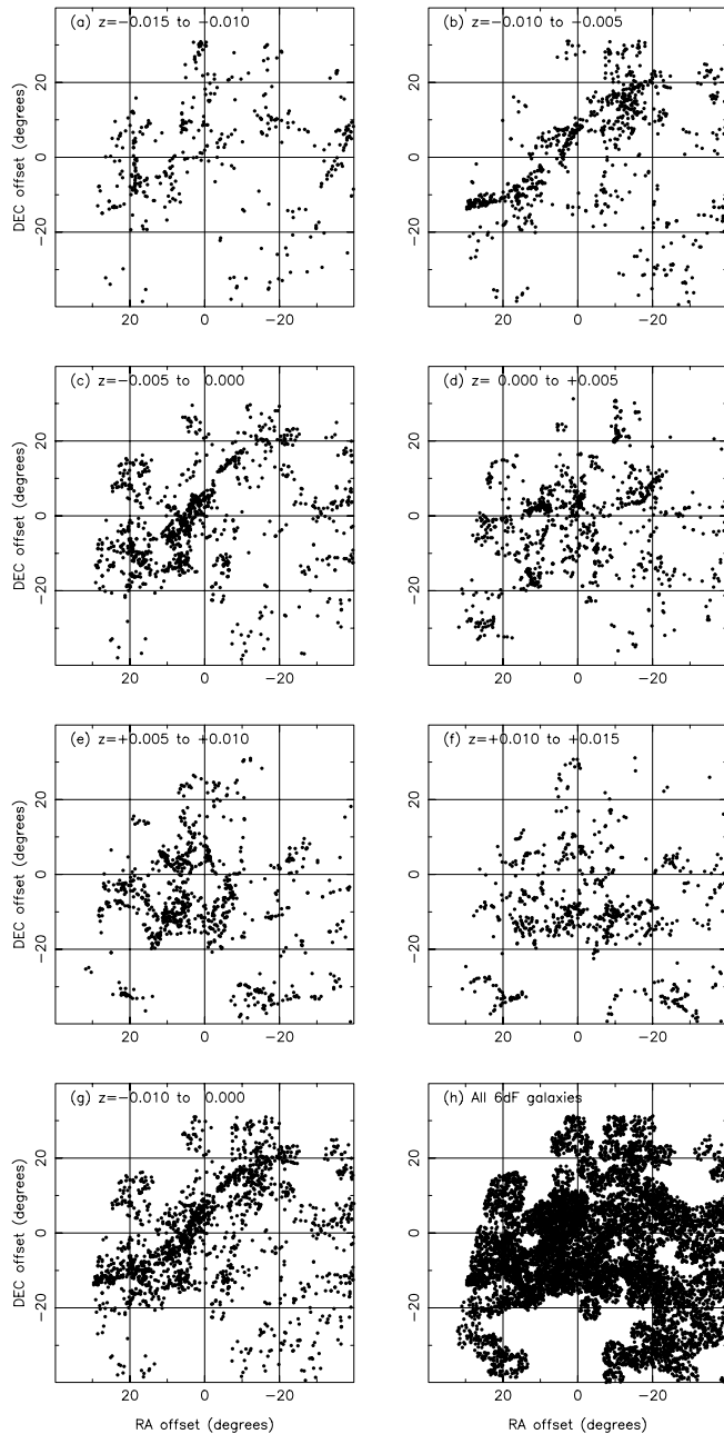
FIG. 7.—Distribution of 6dF galaxies in the vicinity of MSH 05-22; 20^\circ corresponds approximately to a linear distance of 54 Mpc. (a–f) Distribution in redshift slices that are 0.005 wide in redshift space and cover a redshift range \pm 0.015 about that of the host galaxy at z = 0.038286 . (g) All galaxies with redshifts in the range -0.01 – 0.0 relative to the host redshift. (h) All 6dF galaxies in this region with redshifts cataloged to be “reliable” or “probable.”
