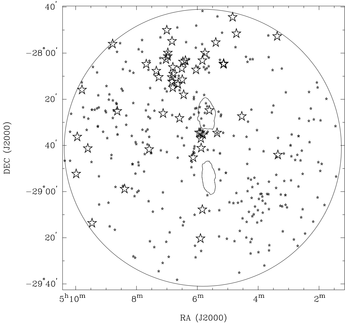
FIG. 9.—Distribution of galaxies close to MSH 05-22; a 20' angular scale corresponds to a linear size of 0.9 Mpc. Galaxies with redshifts in the range z = 0.03\text{--}0.05 are displayed. Large star symbols are for galaxies within \pm 0.003 of the host redshift at z = 0.038286 ; galaxies outside this range are shown with small star symbols. The large circle shows the 1^\circ radius of the 2dF instrument. A contour at 10 \text{ mJy beam}^{-1} shows the lobes of the giant radio source at 843 MHz.
