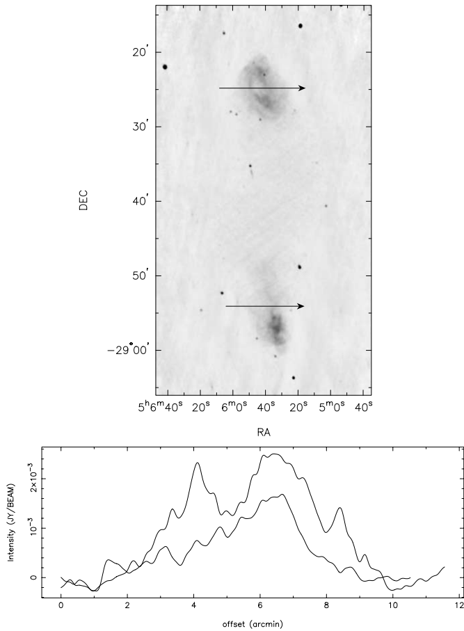
FIG. 10.—Slice profiles across the two lobes of MSH 05-22. The radio image has a beam of FWHM 15.5'' \times 14.2'' at a P.A. of 8.6^\circ .
