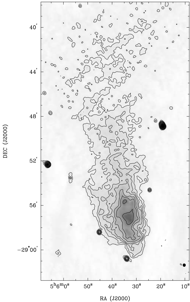
FIG. 3.—The 1520 MHz total intensity VLA image of the southern lobe of MSH 05-22. The beam size, contour levels, and gray-scale range are the same as in Fig. 2.
