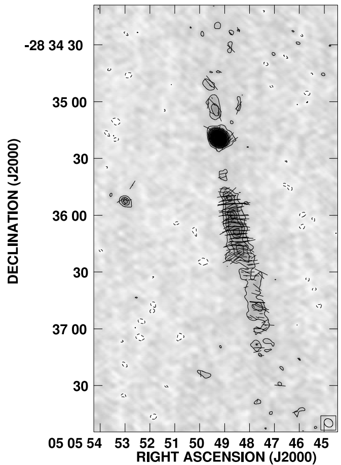
FIG. 6.—The 4860 MHz VLA image of the radio core of MSH 05-22. The radio image has a beam of FWHM 5.0'' \times 4.1'' at a P.A. of 50.8^\circ . The total intensity image is shown using contours and gray scales: contours are at (-1, 1, 2, 3, 4, 6, 8, 12, 16, \text{ and } 32) \times 0.075 \text{ mJy beam}^{-1} , and gray scales are over the range -0.1 to 0.7 \text{ mJy beam}^{-1} . The lowest contour is at 3 times the rms noise. Polarization vectors represent the electric field orientation with length proportional to the polarized intensity: 1'' length corresponds to 10 \mu\text{Jy beam}^{-1} polarized intensity.
