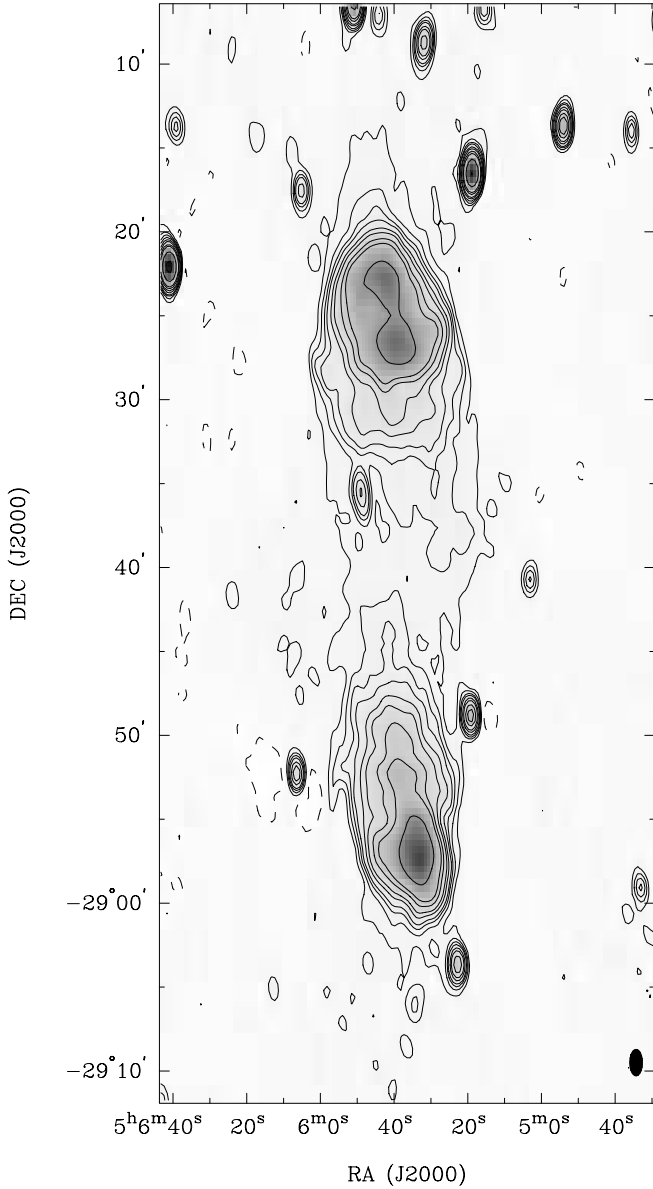
FIG. 1.—The 843 MHz MOST image of MSH 05-22. The radio image has a beam of FWHM 94.0'' \times 45.0'' at a P.A. of 0^\circ and represents the co-addition of several archival images. Contours are at (-1, 1, 2, 3, 4, 6, 8, 12, 16, 32, \text{ and } 64) \times 2.5 \text{ mJy beam}^{-1} ; gray scales are over the range -5 to 200 \text{ mJy beam}^{-1} . The lowest contour is at a level of 3 times the rms noise in the image. In this image, as well as all following images displayed here, the half-maximum size of the beams of the radio images are shown using a filled ellipse in the lower right of the figure. In addition, all the radio images have been corrected for the attenuation due to the primary beam.
