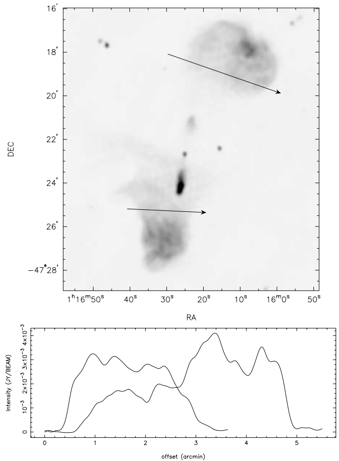
FIG. 11.—Slice profiles across the two lobes of PKS J0116–4722. The radio image has a beam of FWHM 10.24'' \times 9.10'' at a P.A. of 10.7^\circ .
