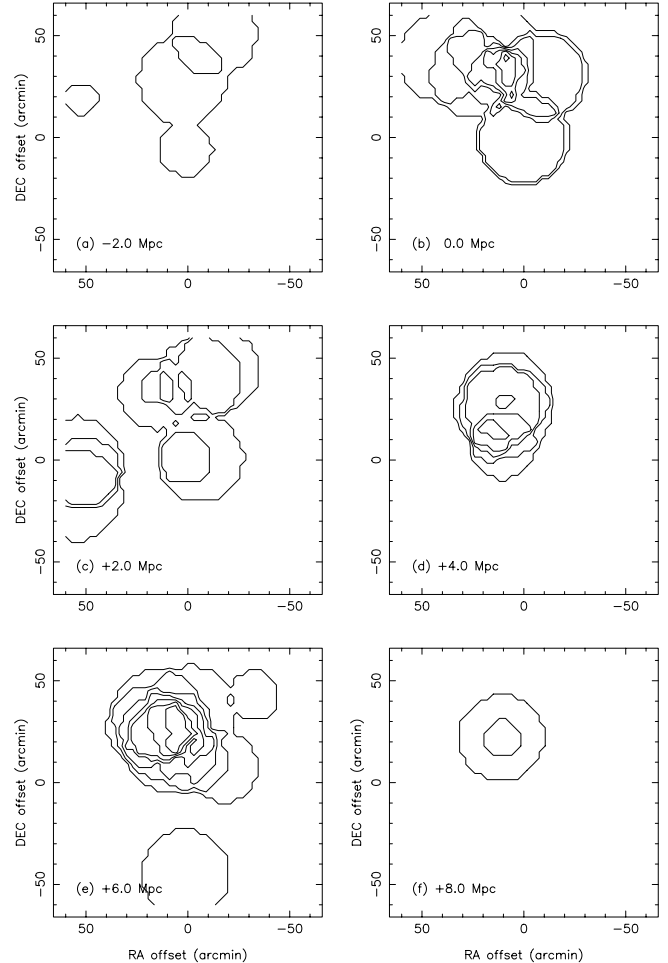
FIG. 13.—Fractional overdensity distribution in the vicinity of MSH 05-22. The 50' angular scale corresponds to a linear size of 2.25 Mpc. Contours are at \Delta n/\bar{n} = 0, 2, 4, 6, 8, 10, and 12 . A spherical top-hat smoothing function with radius R = 1 Mpc was used.
