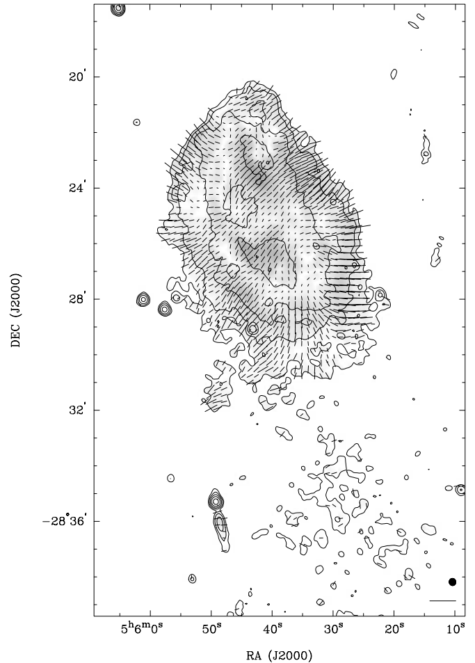
FIG. 4.—The 1520 MHz VLA image of the polarization in the emission from the northern lobe of MSH 05-22. The polarized intensity is displayed using gray scales over the range 0\text{--}4\text{ mJy beam}^{-1} . Contours of the total intensity are overlaid at (-1, 1, 2, 4, 8, 16, \text{ and } 32) \times 0.4\text{ mJy beam}^{-1} . Polarization vectors represent the electric field orientation with length proportional to the fractional polarization. The length of the horizontal bar at the lower right corner of the image represents 100% fractional polarization. The polarization vectors have been corrected for Faraday rotation along the line of sight.
