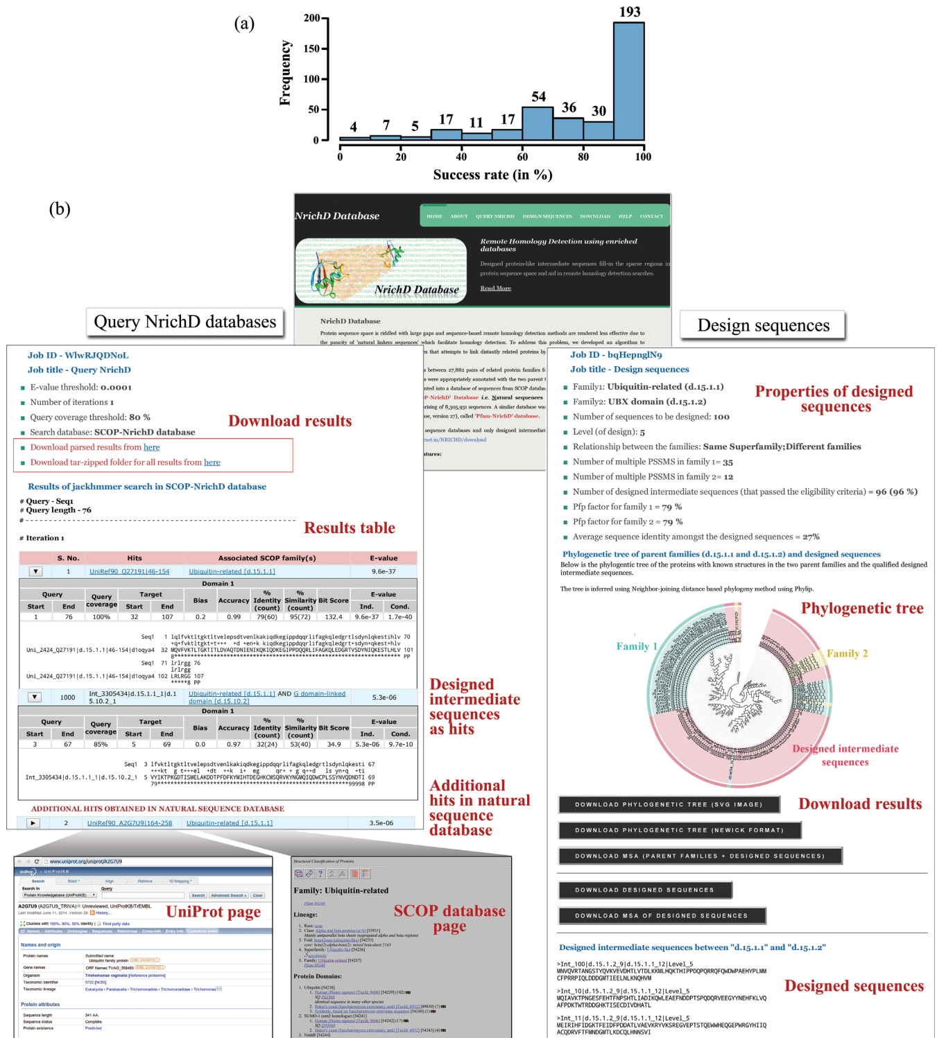
Figure 1. (a). Histogram representation of success rate (in percentage) in designing sequences for 374 folds. (b) Screenshots of Results pages of the database query and protein design interface.
