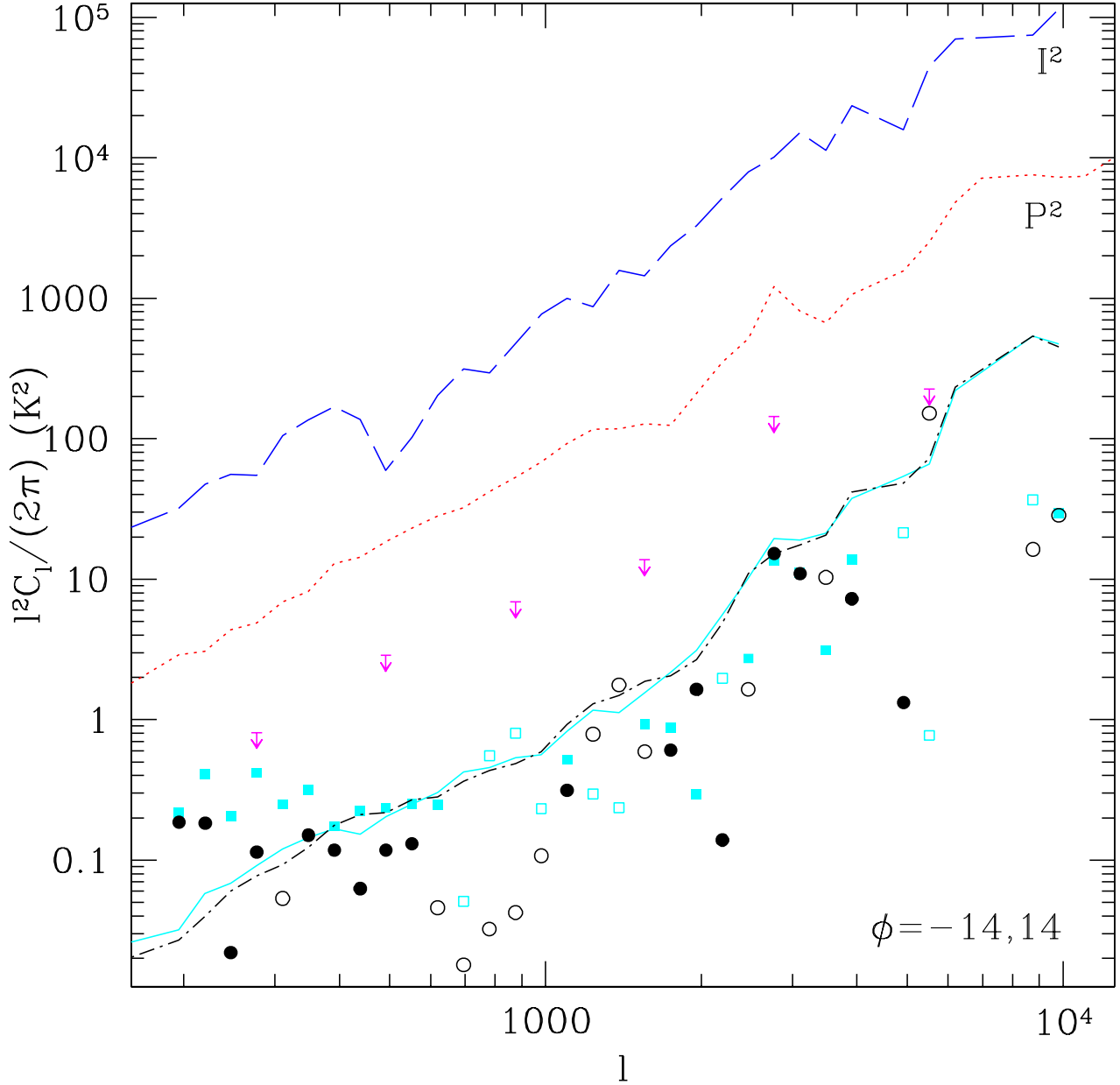
Figure 4. Power spectrum of unpolarized ( I^2 , long dash) and total polarized emission ( P^2 , dotted) over the central square degree, after subtracting the 31 brightest sources in the primary beam. This polarized signal includes leakage and thermal noise. The upper bound symbols are a 2\text{-}\sigma estimate of polarization bound using baseline cross correlation. They are averages of the polarization power in 1 MHz bands. The lower solid and dot-dashed lines are the total power polarization measured at \phi=-14 and 14 over a width \Delta\phi=3.5 , as determined from the map power. Using the cross correlation technique described in the text, we plot a less conservative estimate with circles for \phi = -14 and squares for \phi = +14 . Open symbols denote negative power, and filled are positive values. For details on the unit conversions, see the appendix.
