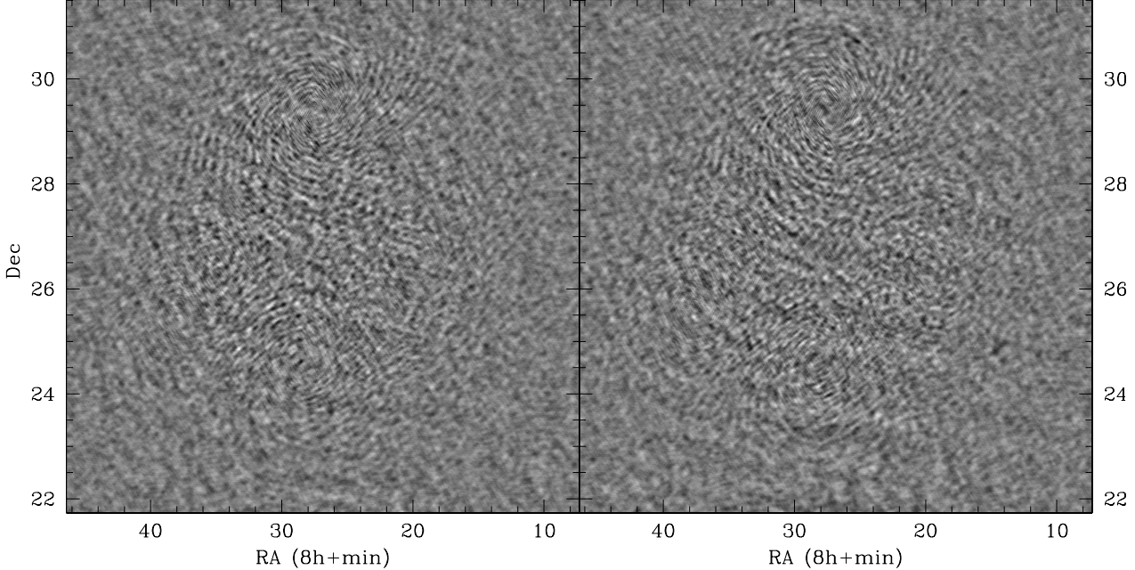
Figure 5. Polarized sky image at \phi = 3 \text{ rad m}^{-2} . The left panel is the Stokes Q intensity, while the right is Stokes U. All baselines with |w| < 200 are included. The field of view is 9.78 degrees, which is three primary beams. Real polarized sky structure as well as leakage I into Q,U will have higher contrast within the main beam region. Sources that generally have the same contrast inside and outside the main beam area include RFI and the aggregate extended image artifacts of multiple bright sources far outside the main beam. These images do show a weak enhancement of contrast in the main beam region, but the enhancement is too weak to allow confidence in detection of sky structure. For this reason we interpret the measured power spectra from these images as upper limits to the polarized sky structure. Artifacts from one known bright source 3C200 are faintly visible as concentric rings centered on the source location. 3C200 is in the upper center of the image just outside the main beam.
