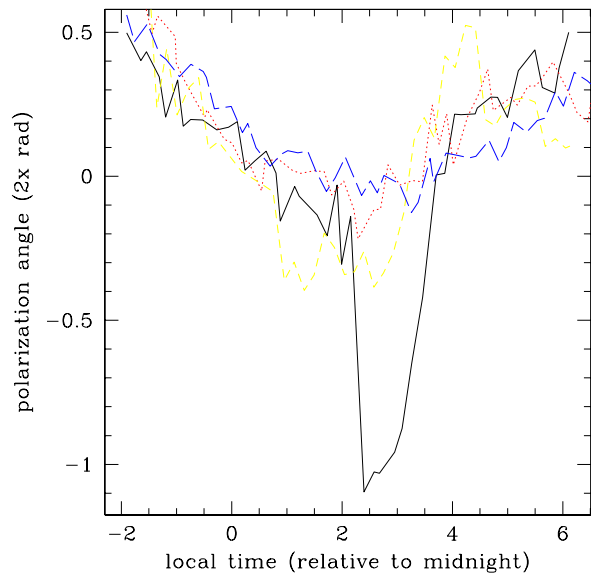
Figure 1. Apparent pulsar polarization angle. The solid, dotted, dashed, long dashed are the mornings of the 18th, 17th, 9th and 16th respectively. The vertical axis is twice the polarization position angle, i.e. \tan^{-1}(U/Q) . The long term change seen in the data (the dip towards the center of the plot) is likely due to change in airmass and geomagnetic field angle, while the variation between each point and those immediately following is consistent with pulsar angle variations at the source. The night of the 18th showed a two hour period in which the polarization angle departed from the slowly changing behavior characteristic of the rest of the data set. This is likely an ionospheric anomaly. For this plot angles are arithmetically averaged over one minute intervals, then the median angle for each 9 minute interval is plotted.
