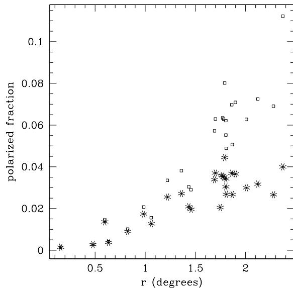
Figure 3. Apparent polarization of sources at Faraday depth \phi=0 \text{ rad/m}^2 . The small squares are the apparent polarizations. The asterisks are multiplied by the primary beam, which is an estimate of their impact to the total polarization in the image. We see that most of the apparent polarized flux contribution is from the periphery of the beam.
