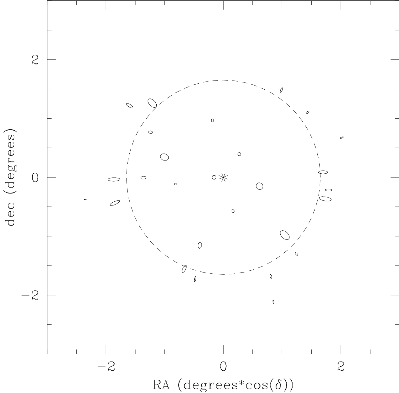
Figure 2. Polarized point source map at Faraday depth \phi = 0 rad/m 2 . The radius (mean of semi-major and semi-minor axes) of each ellipse is proportionate to apparent flux. Ellipticity is proportionate to polarization. Map is averaged over 16 MHz. The asterisk in the center is the pulsar. 5C7.245 has been omitted for clarity. The ellipticity is plotted eight times larger than the apparent polarization. The global polarization angle was rotated to align the pattern radially. The feed support structures could lead to such a polarization pattern (see text). The dashed ring is the half power point of the primary beam. Sources outside that radius appear more strongly polarized.
