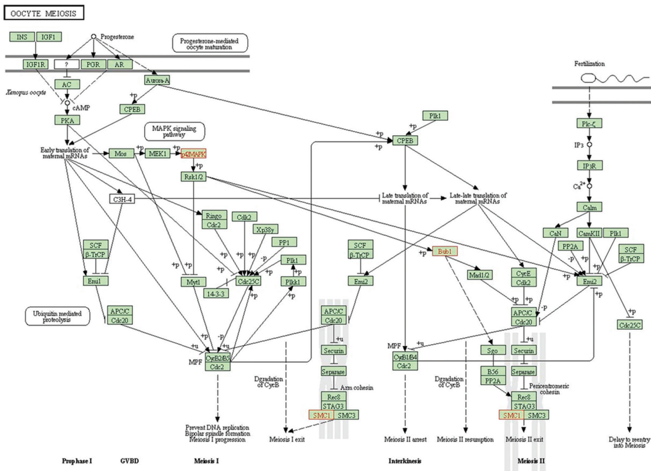
Fig. 3. The KEGG pathway of normal oocyte meiosis. The pathway highlights three copy number variation-enriched genes (mitogen-activated protein kinase, structural maintenance of chromosome 1 and Bub1) indicated in red blocks. The upregulation/downregulation of these genes will affect the normal oocyte pathway. These genes are identified in the major steps i.e. , meiosis I and meiosis II.
