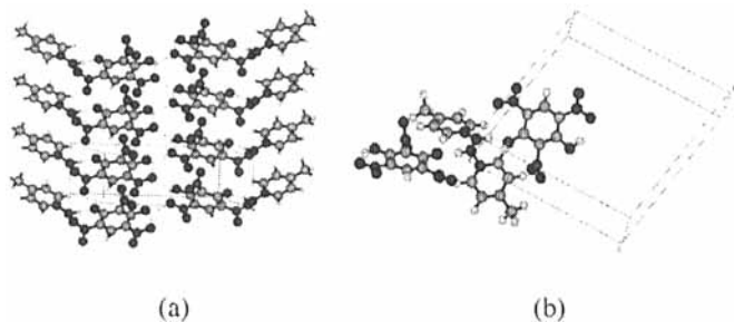
FIGURE 2: Herringbone motif (a) and quasi tetrahedral motif (b) in 1-hydroxy-4-methylpyridinium 3-hydroxy-2,4,6-trinitrophenolate
