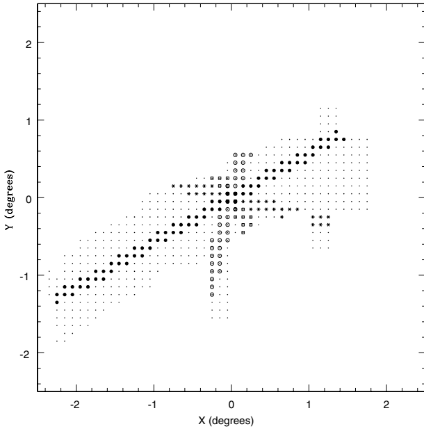
Fig. 3. The locations used to estimate the number density distribution of RRLS as shown in Fig. 2, where PA = 120° (along the bar, filled circle), 75° (asterix), 165° (open circle) and 210° (across the bar, open square). The small dots indicate spatial coverage of the OGLE II survey.
