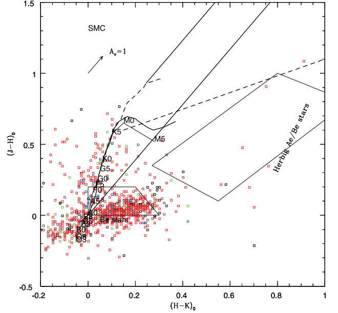
Figure 4. NIR colour-colour diagram of the Be candidates in the SMC (same colour code as in Fig. 1), rest same as Fig. 3.
