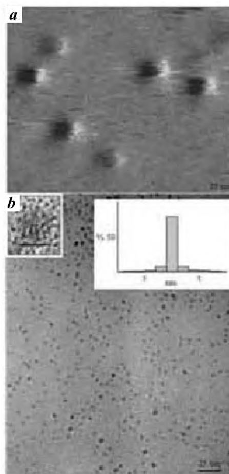
Figure 2. a , STM image of polymer-coated \text{Pd}_{561} nanocrystals. The nanocrystals are seen as fluffy balls against plane background of the graphite substrate. The image was acquired with a bias voltage of 750 mV and a feedback current of 1 nA; b , TEM micrograph showing isolated \text{Pd}_{561} nanocrystals. Histogram in the inset shows the distribution in the diameter. The characteristic 11[111] fringes and the icosahedral shape of an individual metal core can be seen clearly in the high-resolution micrograph shown in the inset. The diameter of the nanocrystals estimated from STM and TEM are ~3.4 and 2.5 nm respectively, the difference being due to the ligand shell, PVP.
