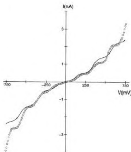
Figure 3. I – V characteristics of an isolated Pd 561 nanocrystal (dotted line) obtained at 300 K using a STM set up. The nanocrystals were first dispersed on a highly oriented pyrolytic graphite (HOPG) substrate by drop casting. The theoretical fit (solid line) using a semiclassical model is also shown. The fit yielded capacitance: C_1 = 0.07 \text{ aF} , C_2 = 0.7 \text{ aF} and resistance: R_1 = 0.5 \text{ M}\Omega , R_2 = 255 \text{ M}\Omega .
