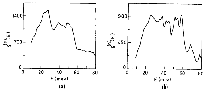
Figure 2. Neutron-weighted phonon density of states for (a) Tl-2122 and (b) Y-123 for Q = 6 \text{ \AA}^{-1} . The energy resolution varied from 5 to 25 meV in the range of E from 0 to 80 meV.
