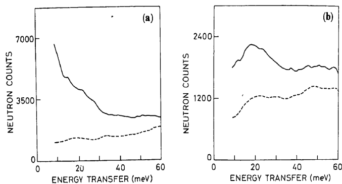
Figure 1. Observed neutron intensity from (a) Tl-2122 and (b) Y-123, with E_f and Q held constant at 30 meV and 6 \text{ \AA}^{-1} respectively. Continuous and dashed lines show raw data and background contribution respectively.
