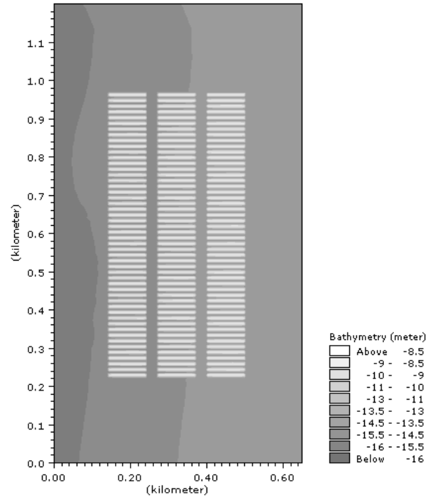
Fig.2 Bathymetry map with tanks of smaller domain of grid size 5mx1m
