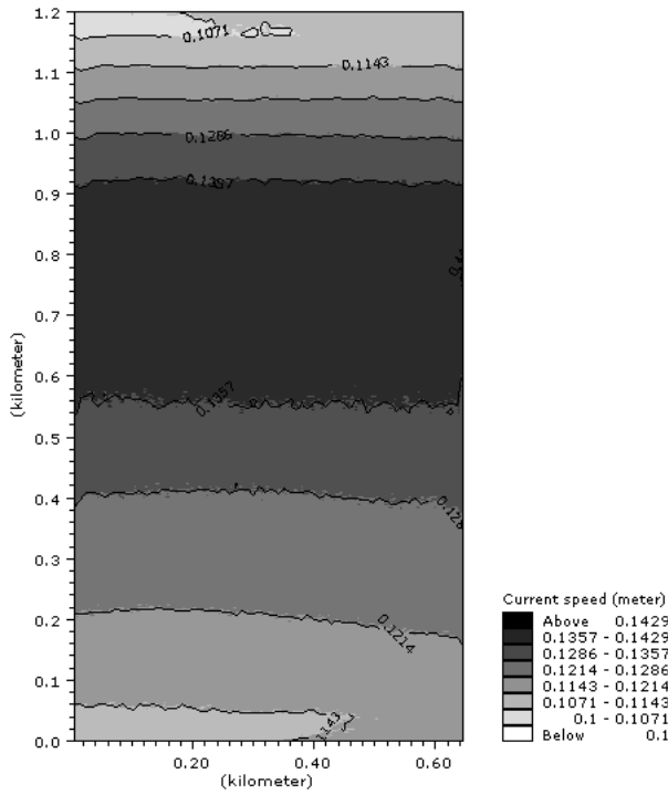
Fig.6a Maximum currents of pre-tanks condition for flood tide phase
